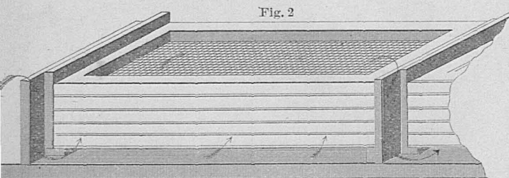
Nest of trays in Williamson's Double Riffle Hatching-Box.
