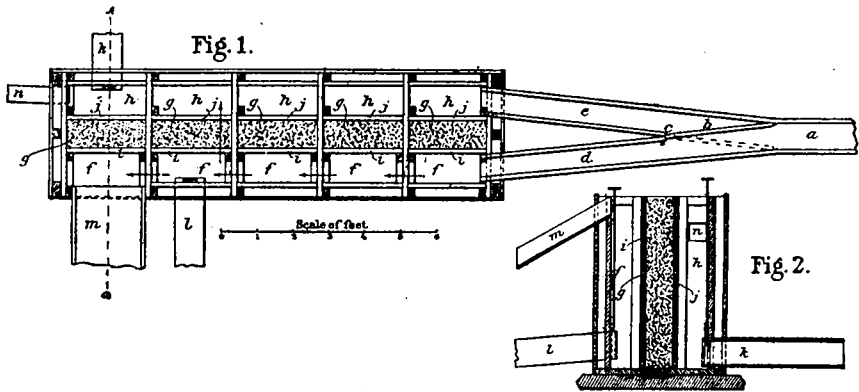
Gravel Filter.
