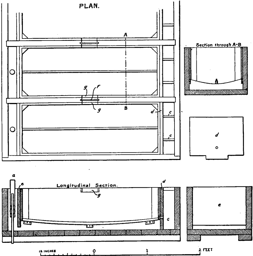
Diagram of Tidal Cod Hatching-Box.
