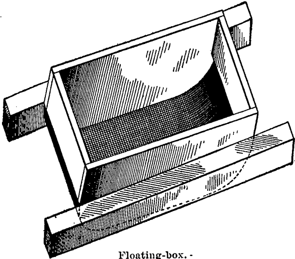
Floating-box. -
