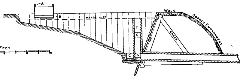
REARING POND.
