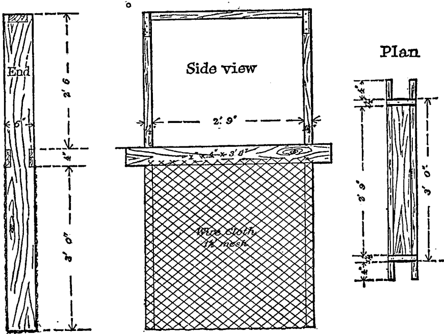
CUT 6.—Receptacle for culch.
