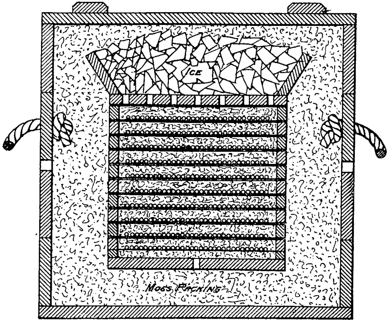
Cross-section through Box after it has been packed and closed.
