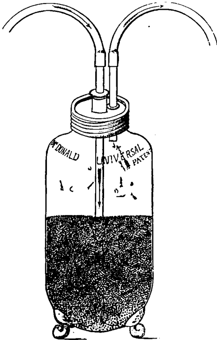
Automatic shad-hatching jar.
