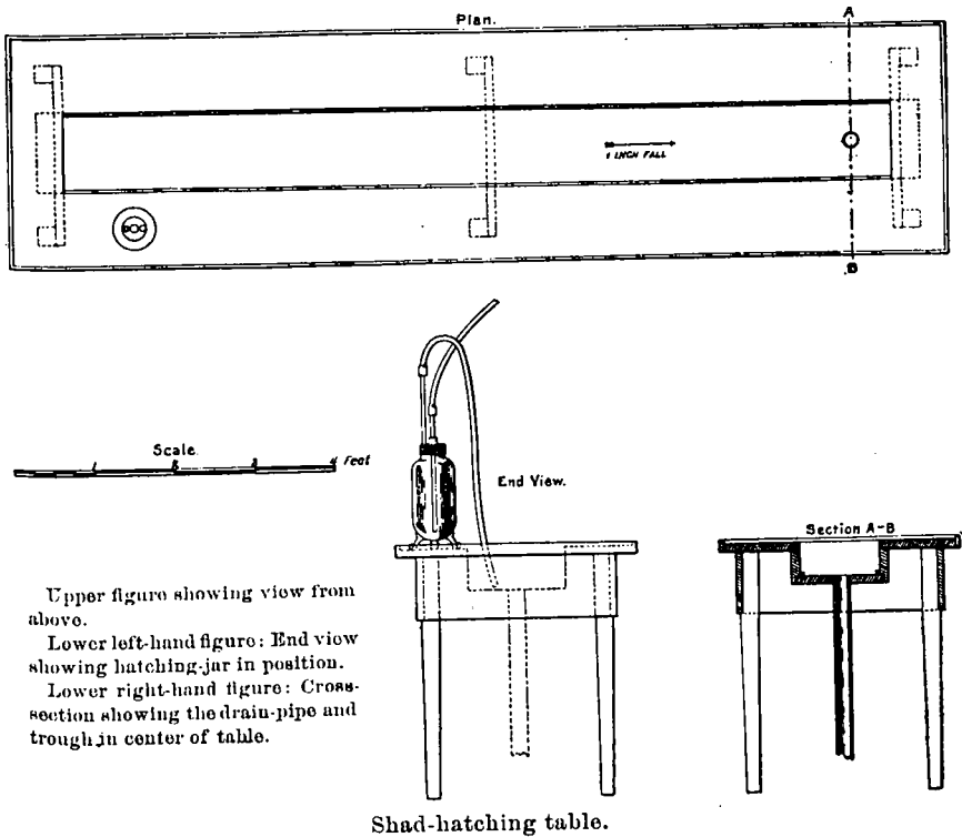
Shad-hatching table.
