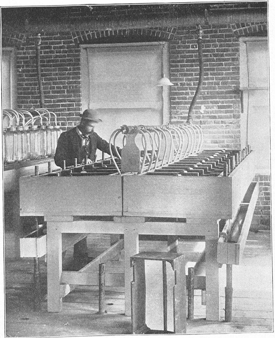
McDONALD TIDAL BOXES, USED FOR HATCHING COD AND FLATFISH.
