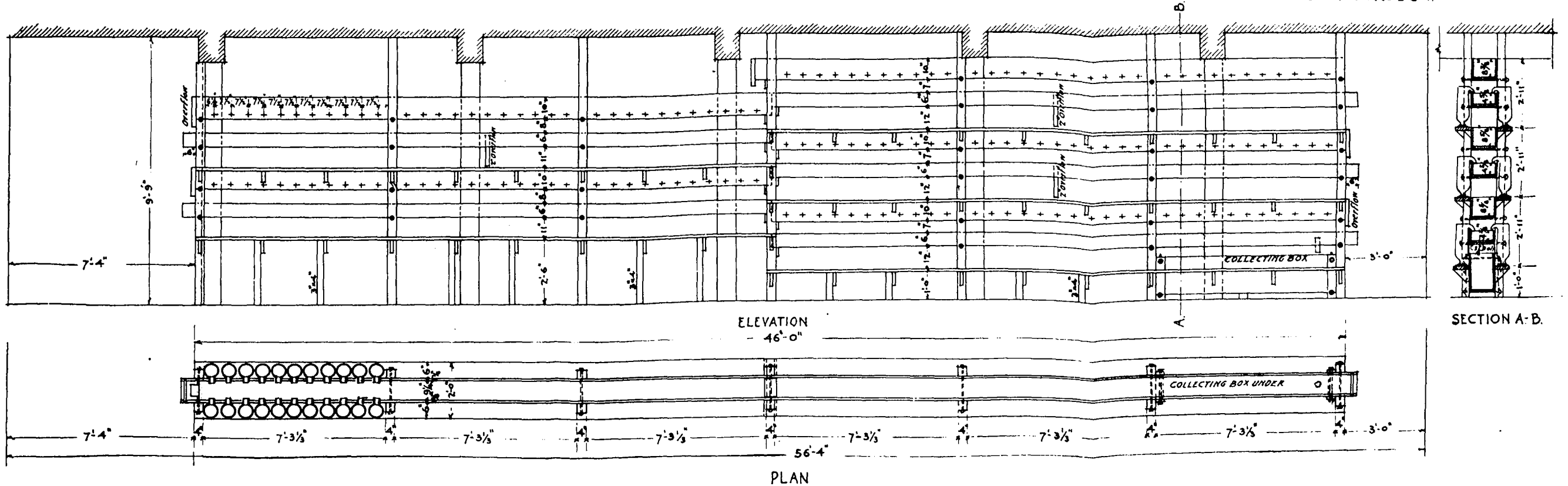
FIG. 1.—Plan of hatching battery in use at the Cape Vincent (N. Y.) station for the incubation of whitefish and cisco eggs. (Designed by J. P. Snyder.)
