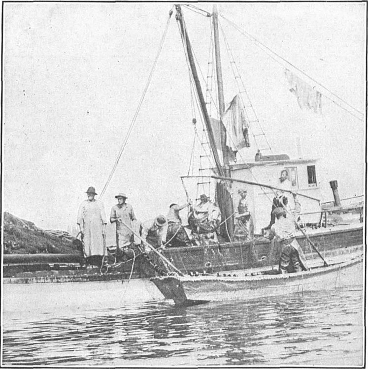
FIG. 17.—DIPPING SALMON FROM A PURSE SEINE.
