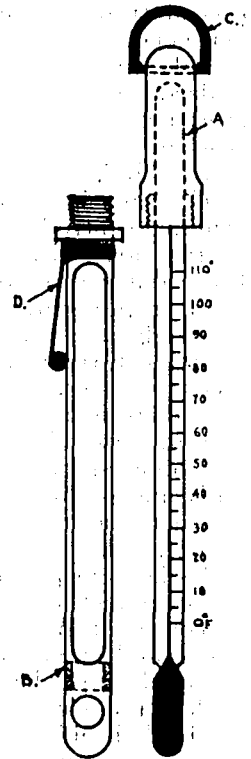
FIG. 5.—Pocket thermometer designed particularly for use in connection with the distribution of living fishes. (Designed by E. C. Fearnow.)
