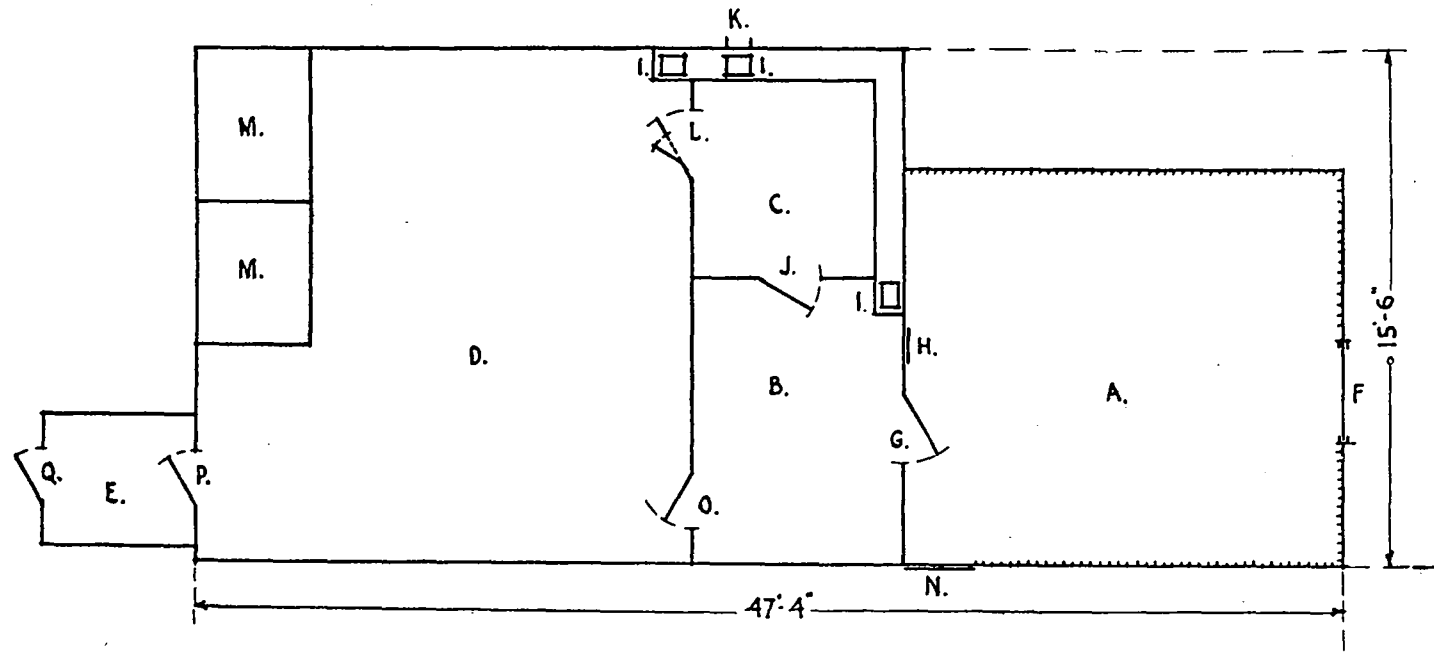
FIG. 1.—INTERIOR ARRANGEMENT OF FOX-TRAPPING HOUSE.
