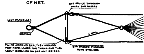
DETAIL OF TOWING END OF NET.
