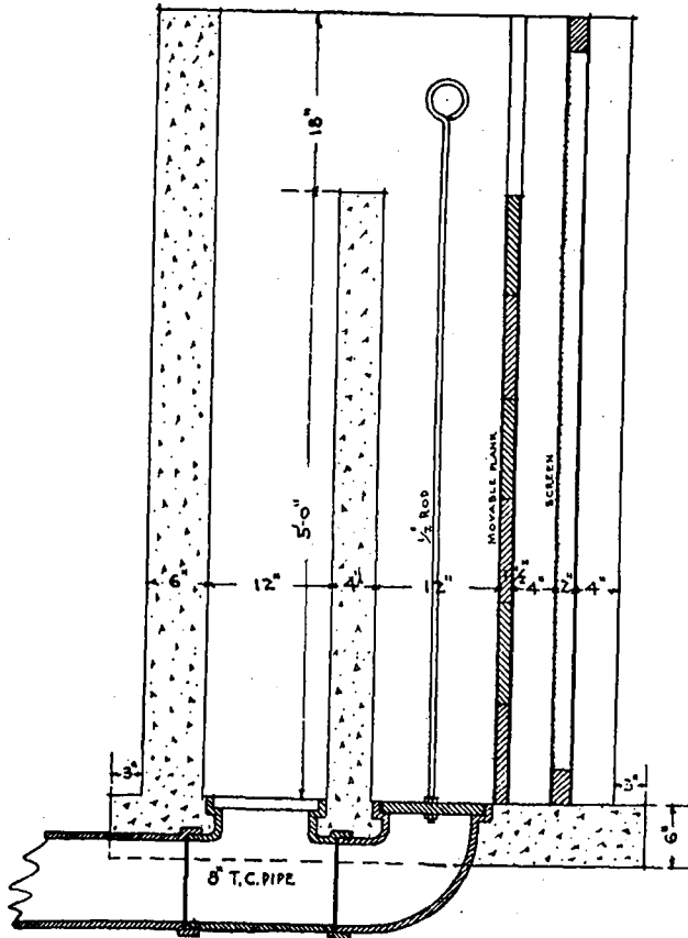
SECTION
