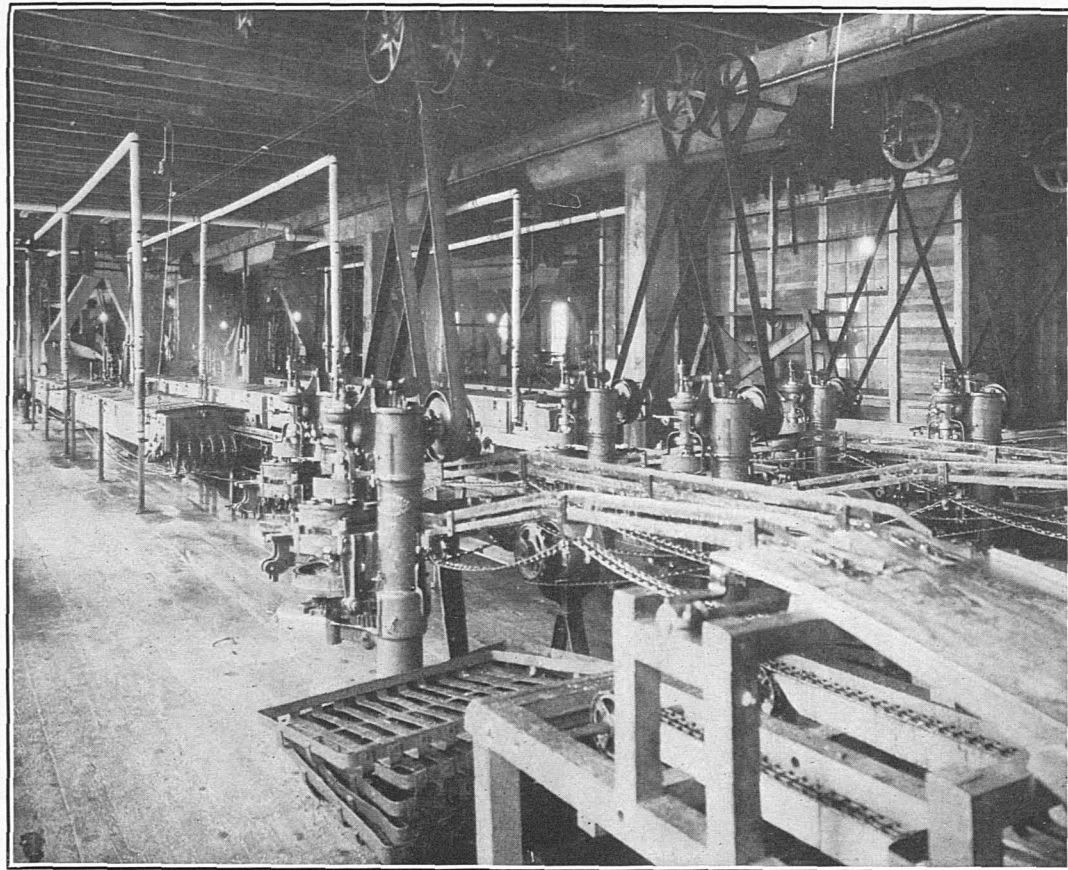
FIG. 30.—EXHAUST BOXES AND THE DOUBLE SEAMERS.
