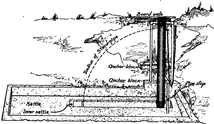
FIG. 2.—The Canfield pond outlet, end view.
