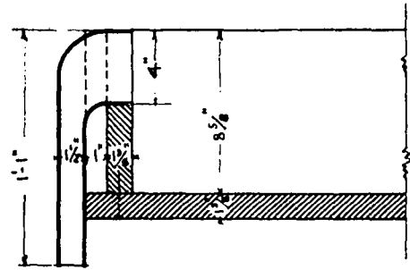
LONGITUDINAL SECTION THROUGH SUPPLY TROUGH
