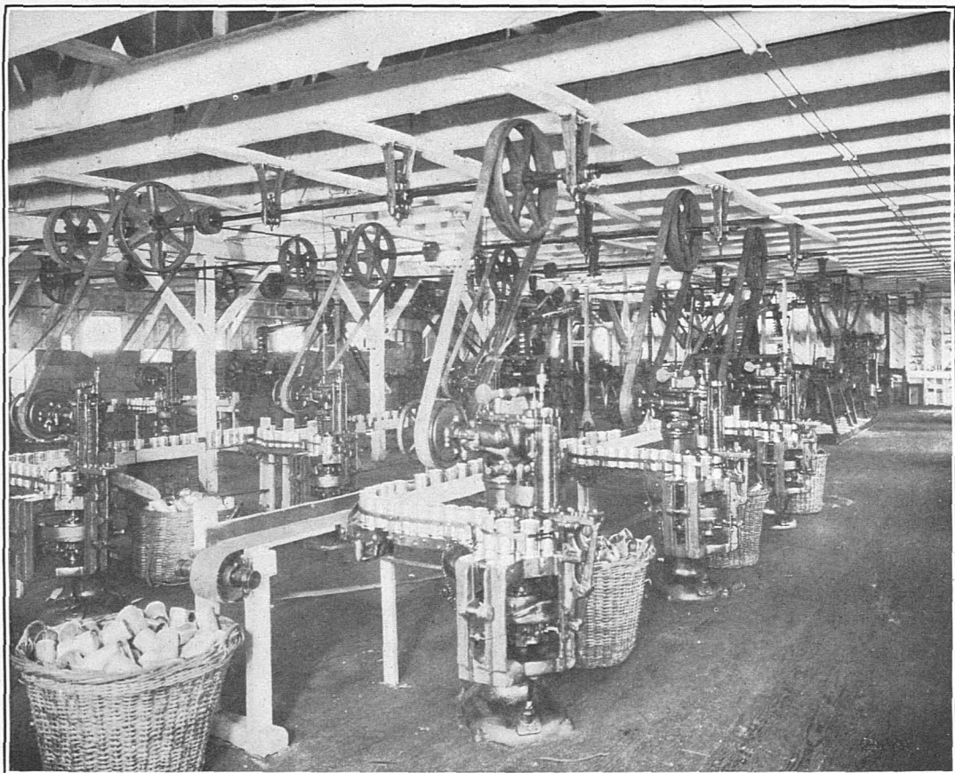
FIG. 35.—MAKING SALMON CANS.
