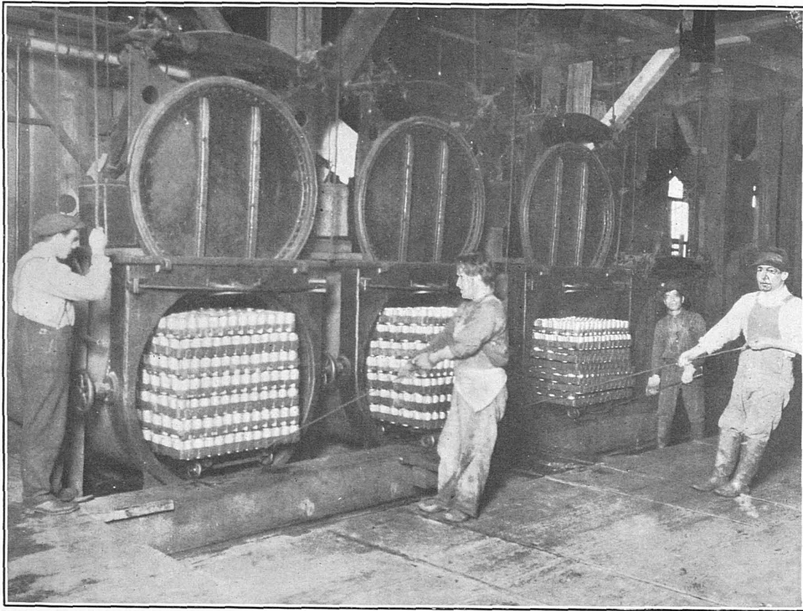
FIG. 31.—COOKING THE SALMON IN RETORTS.
