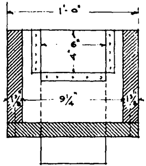
CROSS SECTION THROUGH SUPPLY TROUGH
