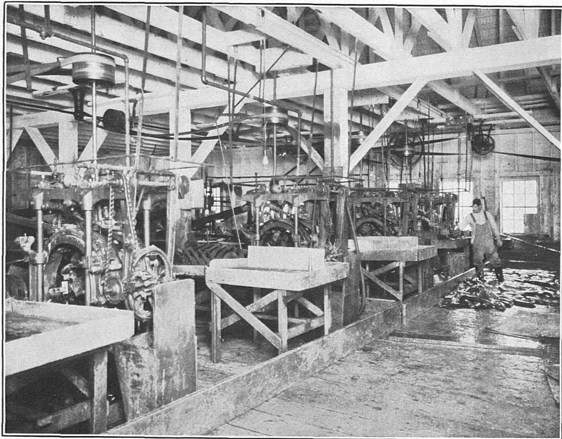
FIG. 28.—A BATTERY OF "IRON CHINKS."
