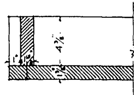
LONGITUDINAL SECTION THROUGH DRAIN TROUGH
