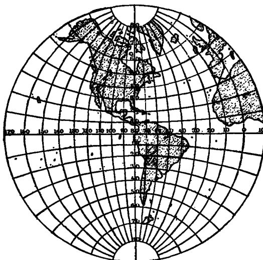
FIG. 31.—Stereographic projection of the Western Hemisphere.
