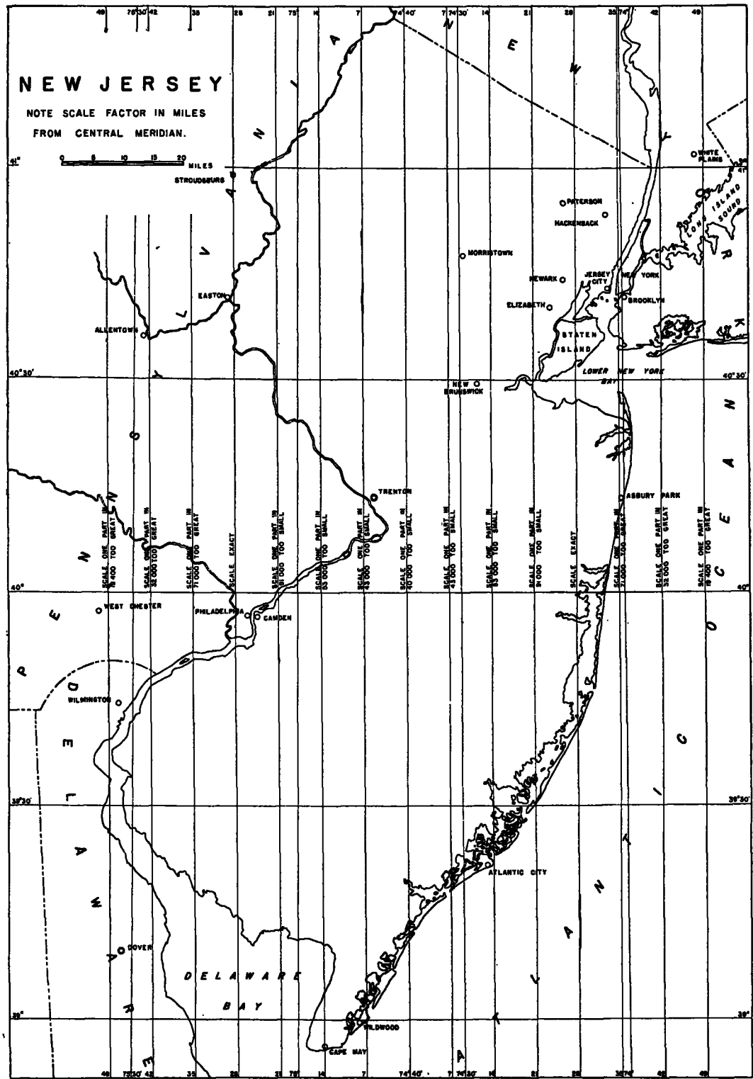
FIG. 88.—Transverse Mercator projection for rectangular coordinates.
