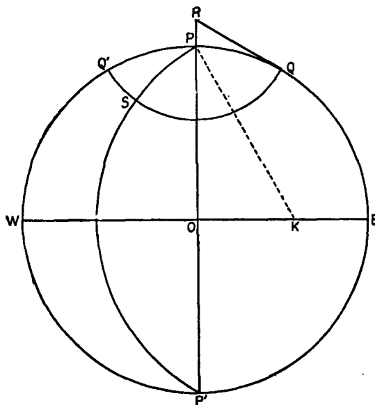
FIG. 36.—Determination of the elements of a stereographic projection on the plane of a meridian.
