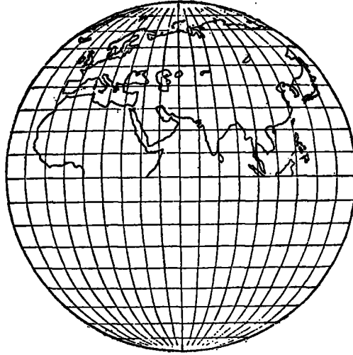
FIG. 77.—The Mollweide homalographic projection of a hemisphere.
