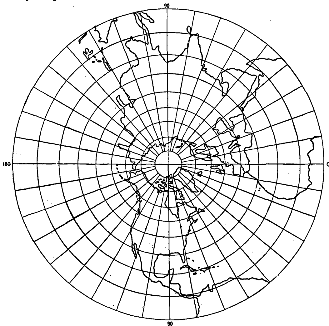
FIG. 23.—Stereographic polar projection.
