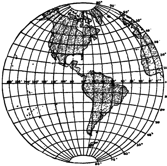
FIG. 33.—Lambert equal-area projection of the Western Hemisphere.
