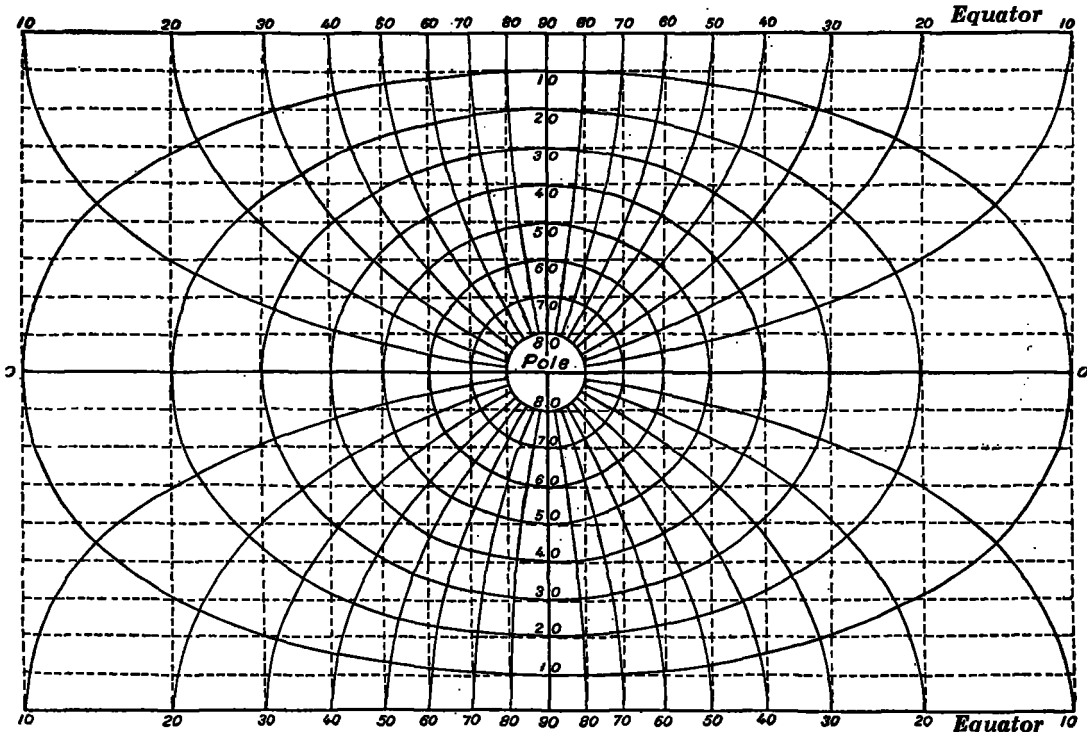
FIG. 64.—Transverse Mercator projection, construction plate.
