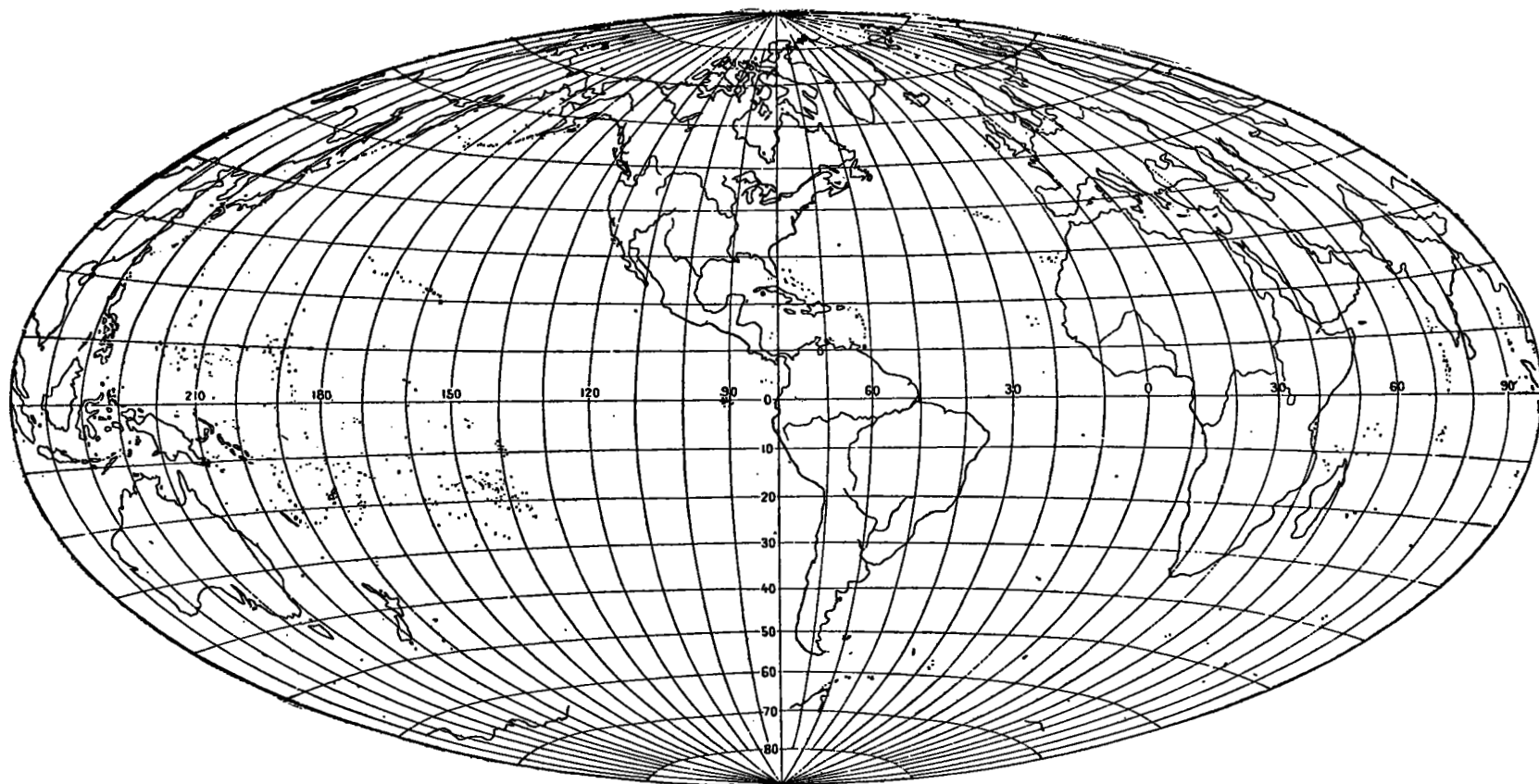
FIG. 75.—The Aitoff equal-area projection of the sphere with the Americas in center.
