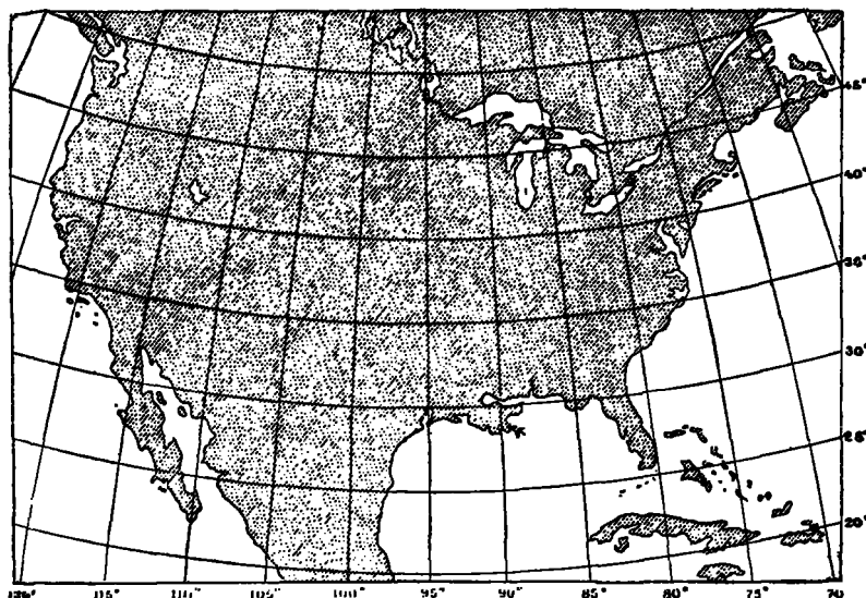
Fig. 41.—Bonne projection of the United States.
