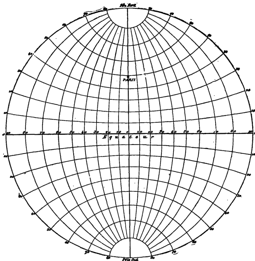
FIG. 73.—Stereographic meridional projection.
