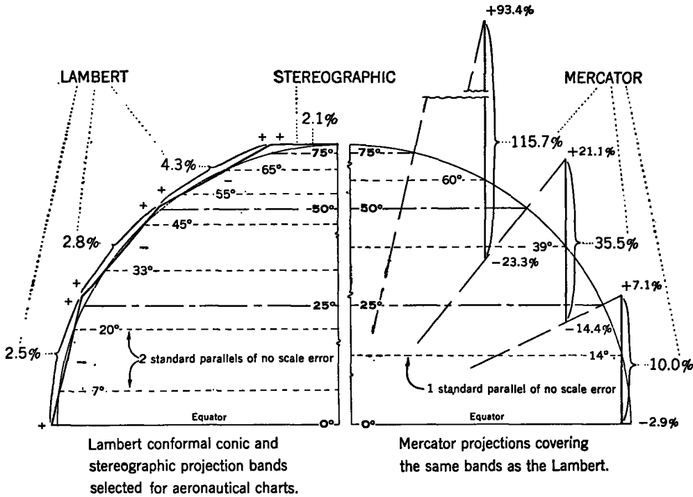
FIG. 85.—Variation in scale of each projection band.
