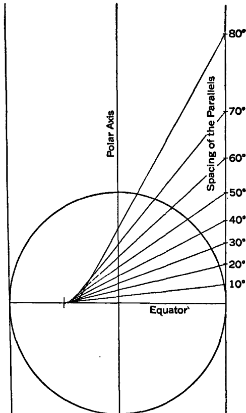
FIG. 21.—Mercator projection showing spacing of the parallels.
