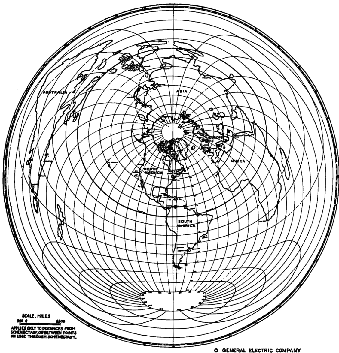
FIG 82 -- AZIMUTHAL EQUIDISTANT PROJECTION OF THE WORLD
