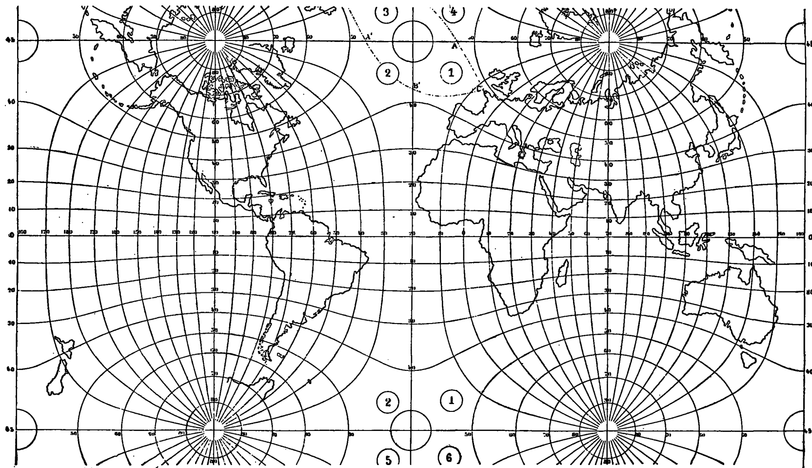
FIG. 79.—Guyou's doubly periodic projection of the sphere.
