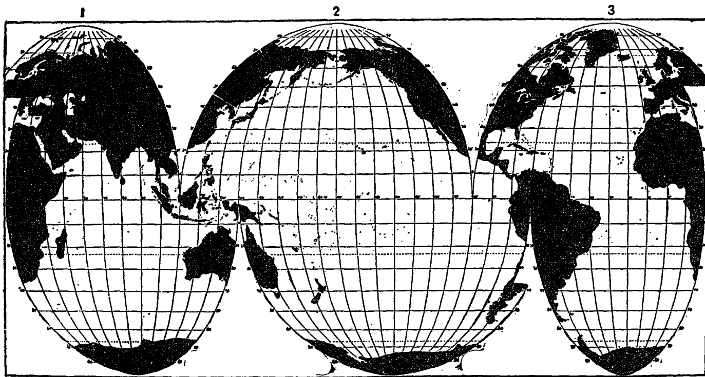
FIG. 78.—Homalographic projection (interrupted) for ocean units.
