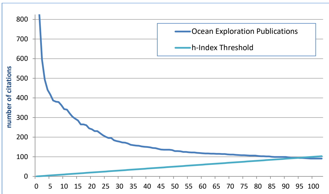
Figure 8: Distribution curve showing the citation counts of the 103 most highly cited publications supported by Ocean Exploration. The straight line indicates the h -Index threshold (slope: y = x ). The intersect point of the two curves ( x = 94 ) is the h -Index of Ocean Exploration articles.
