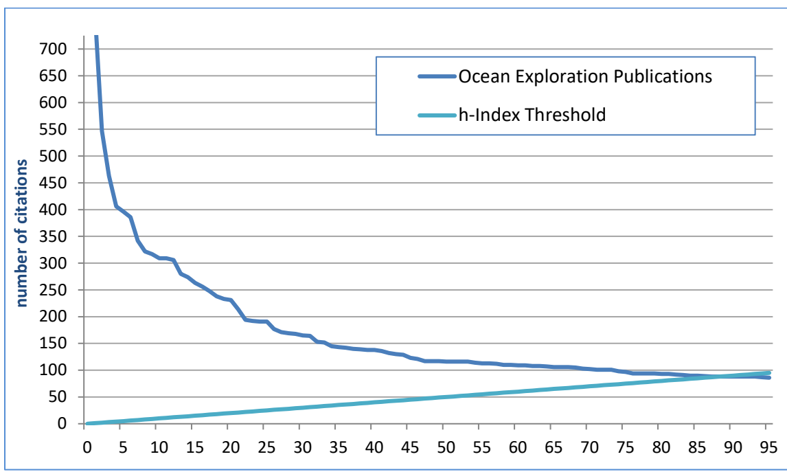
Figure 8: Distribution curve showing the citation counts of the 95 most highly cited publications supported by Ocean Exploration. The straight line indicates the h -Index threshold (slope: y = x ). The intersect point of the two curves ( x = 88 ) is the h -Index of Ocean Exploration articles.
