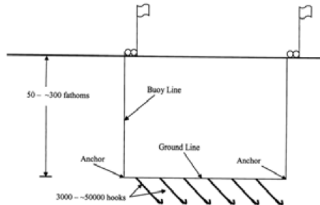
Figure 7-1: Typical Longline Configuration
