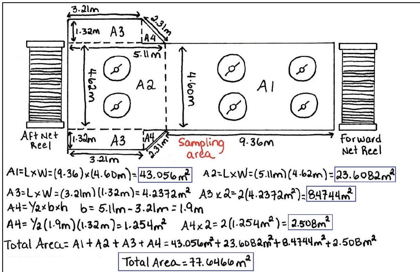
Figure 4-6: Calculating Area of an Irregular Shaped Trawl Alley
