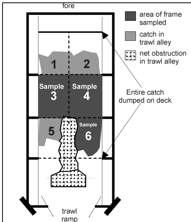
Figure 5-1: Spatial Design Using Trawl Alley
