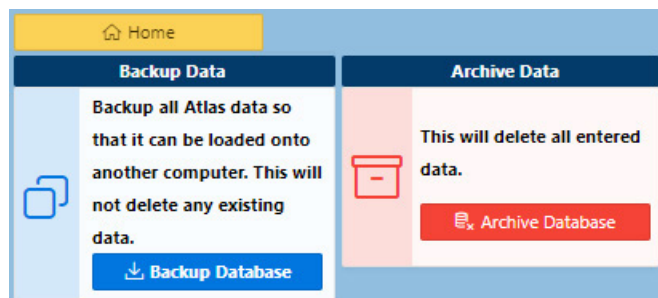
Figure 18-76: Backup/Archive Screen
