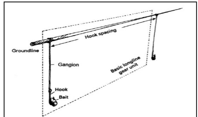
Figure 7-7: Hook Spacing
