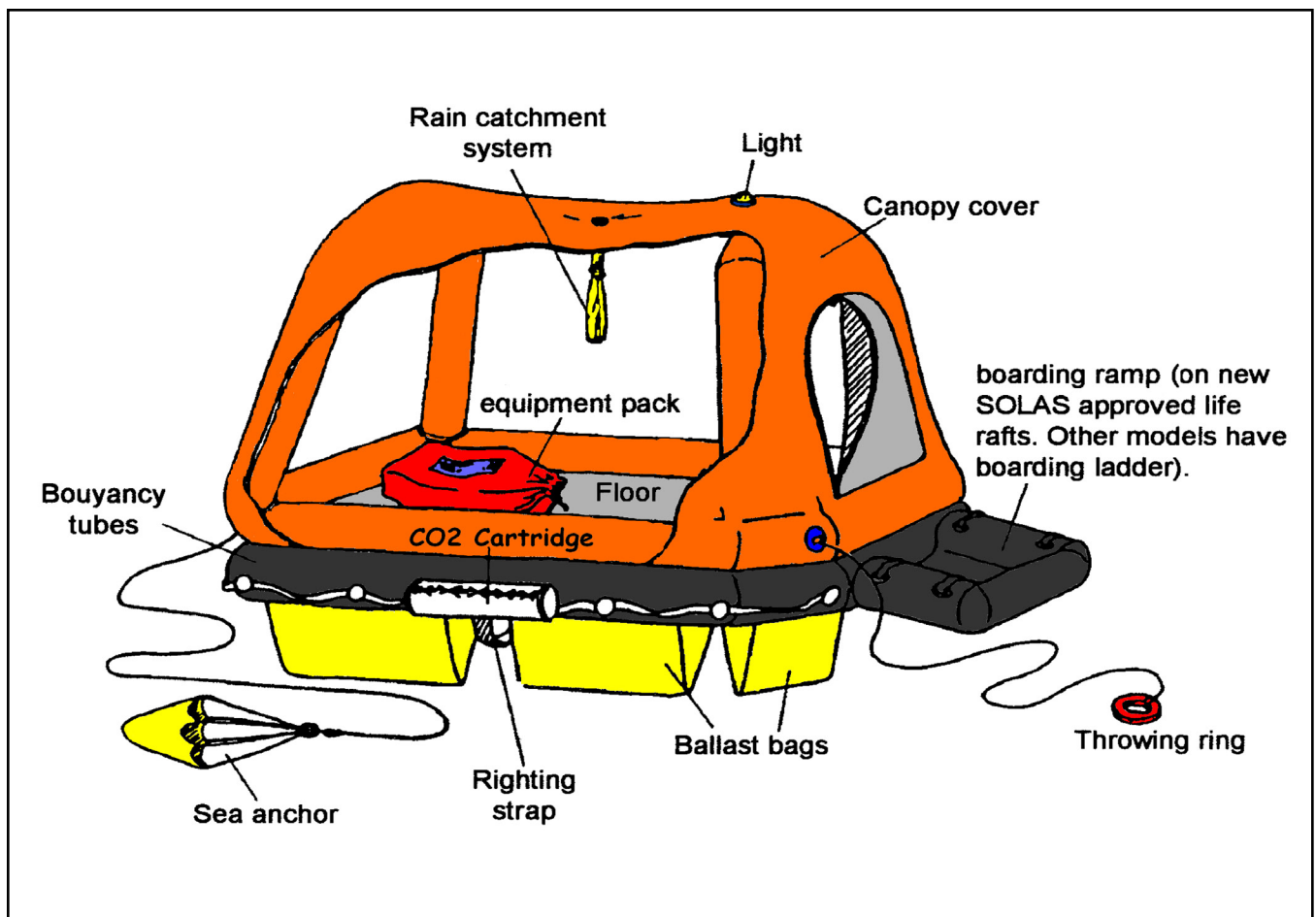
Figure 19-2: Life Raft and Equipment
