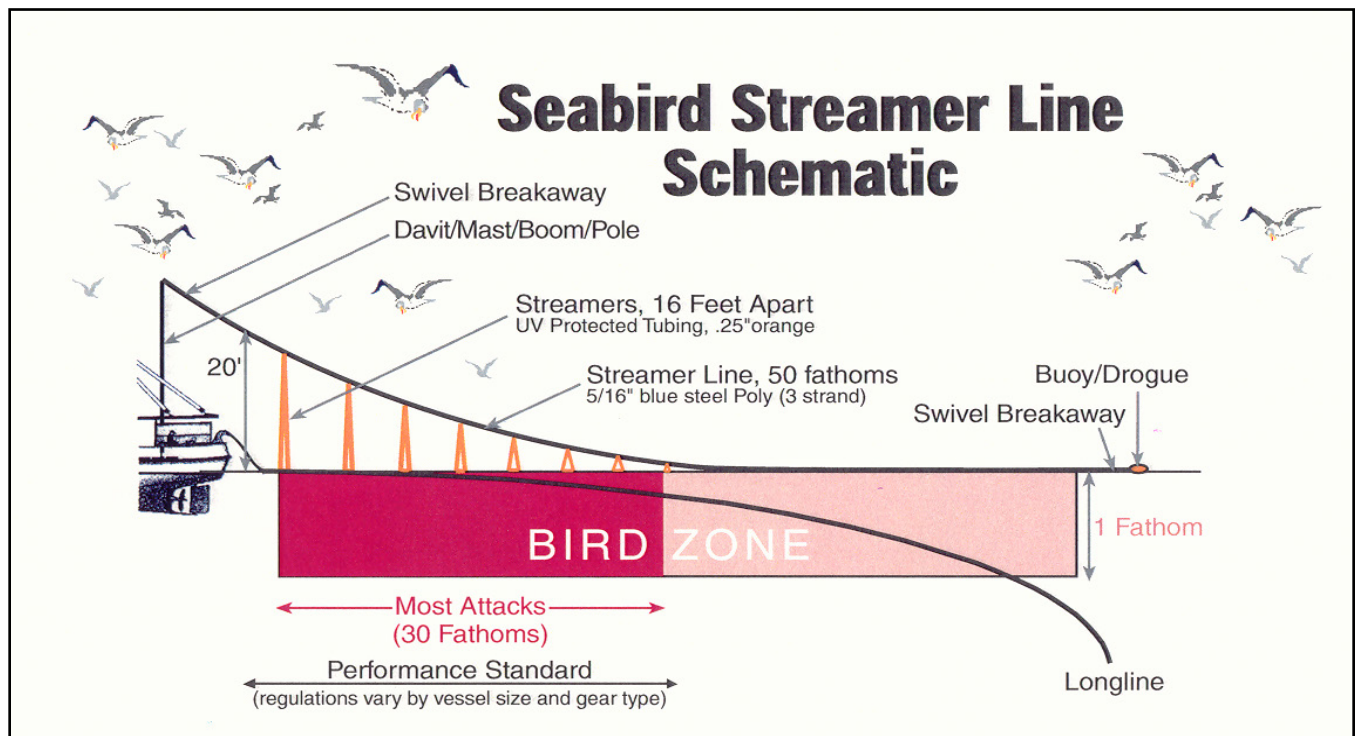
Figure 7-6: Seabird Steamer Line Schematic
