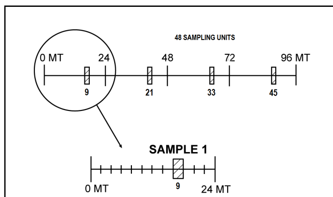
Figure 5-4: Small Systematic Samples on a Vessel with a Flow Scale and High Species Diversity
