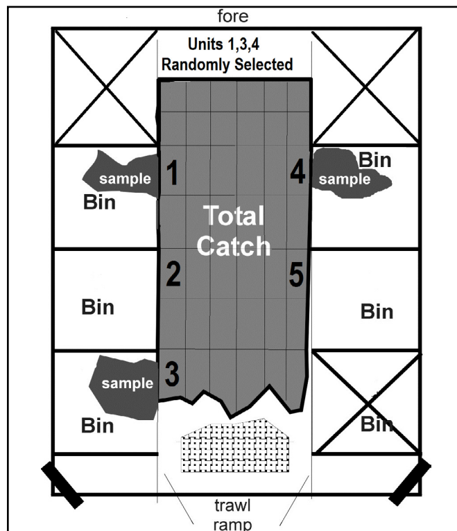
Figure 5-2: Spatial Design Using Checker bins
