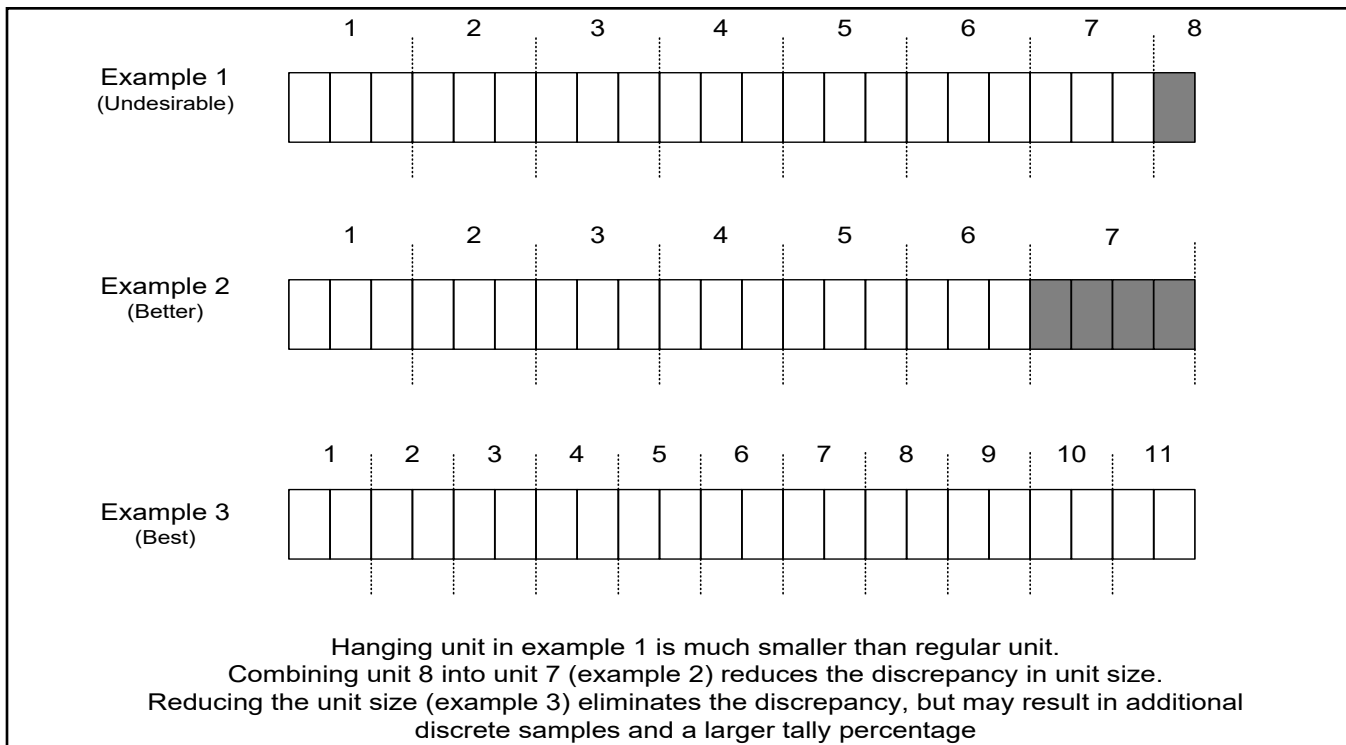
Figure 8-1: Minimizing Size Discrepancy with Hanging Units
