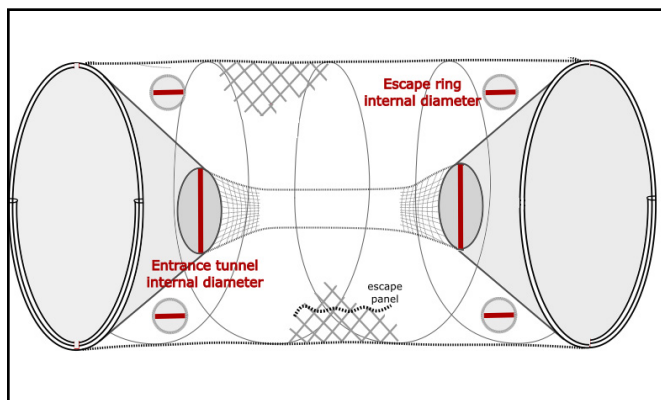
Figure 9-3: Slinky Pot Entrance Tunnel and Escape Ring Pot Opening Measurements Diagram
