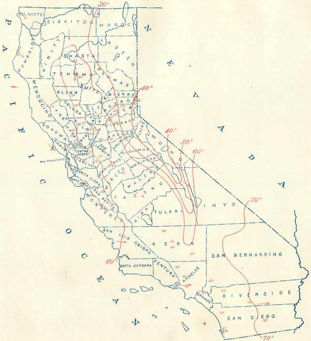
Mean Annual Isotherms and Prevailing Winds. Based on 20 years' normals.
