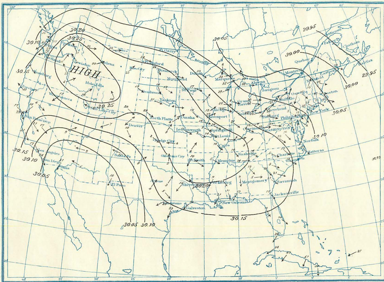
Sea-Level Pressure ; Resultant Surface Winds. January, 1902.
