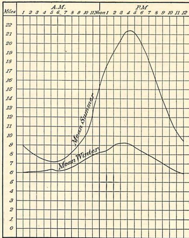
FIG. 7.—Hourly wind velocities at San Francisco.
