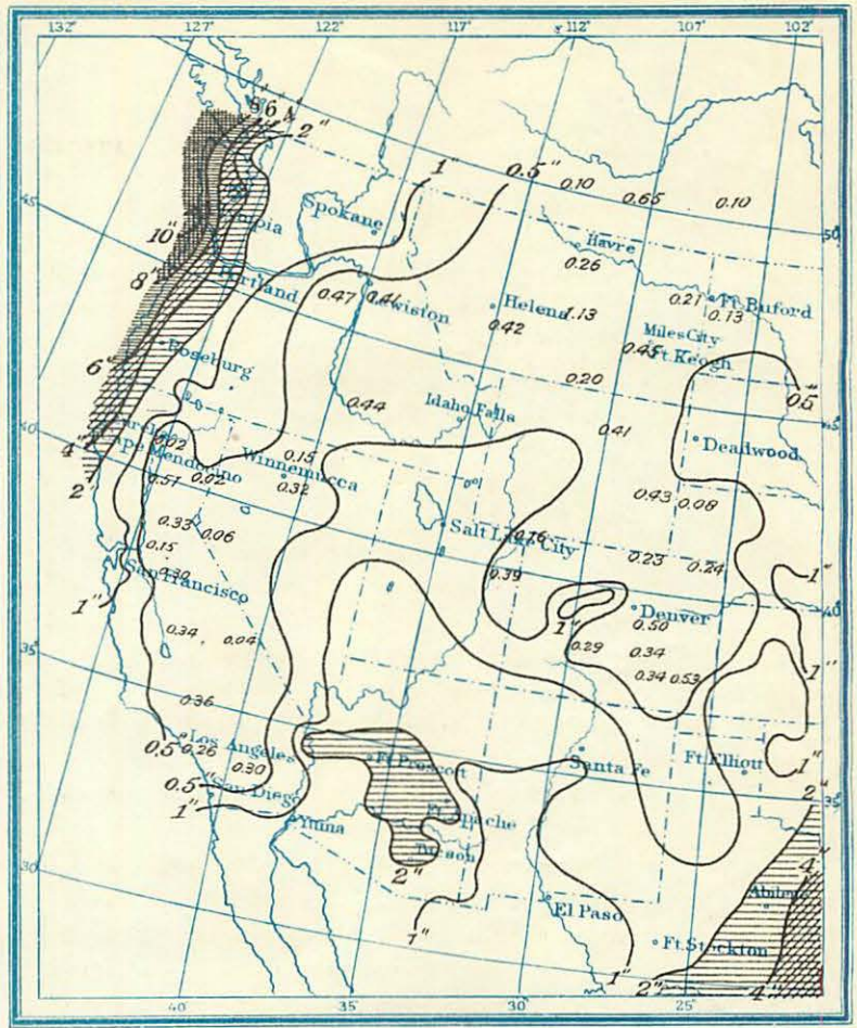
Pressure, Wind, and Rainfall during a Dry winter month.—January, 1889.
