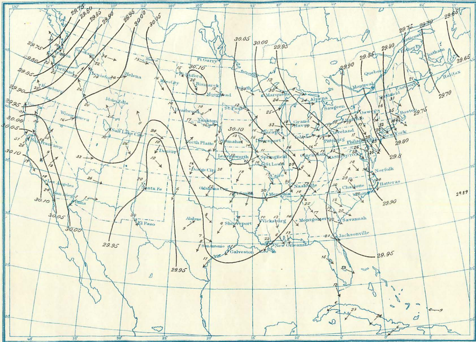
Sea-Level Pressure; Resultant Surface Winds. February, 1902.
