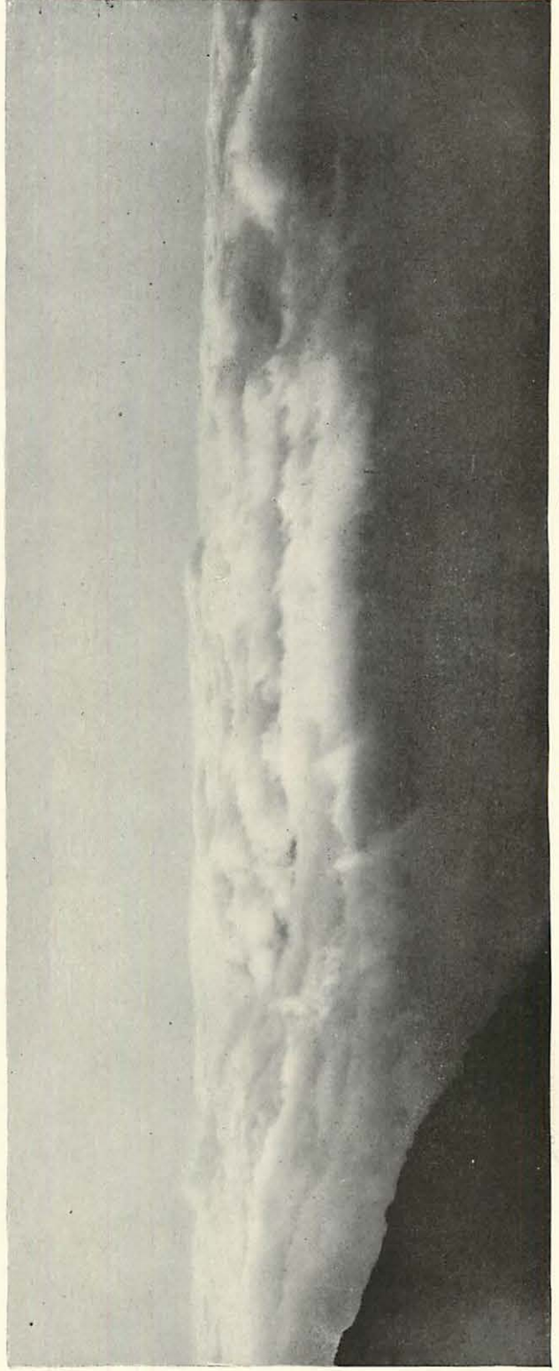
FIG. 22.—LIFTED FOG. HEIGHT ABOVE GROUND ABOUT 500 METERS.
