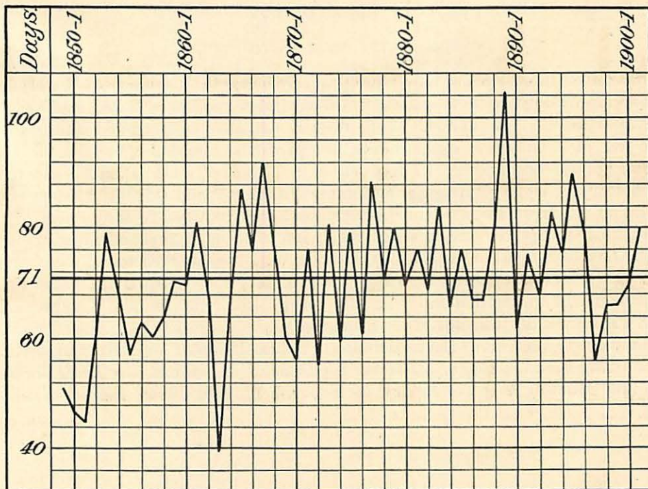
FIG. 3.—Seasonal rainfall at San Francisco, Cal. Frequency, or number of days. (Average, 71 days.)
