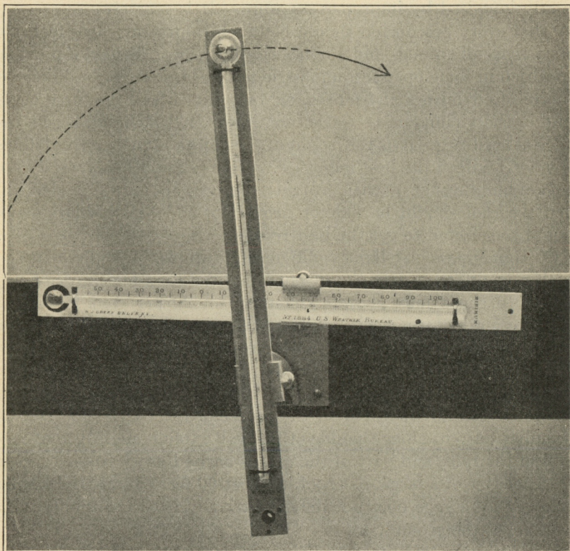
FIG. 10.—Thermometer supports. Pawl disengaged, maximum rotating.
