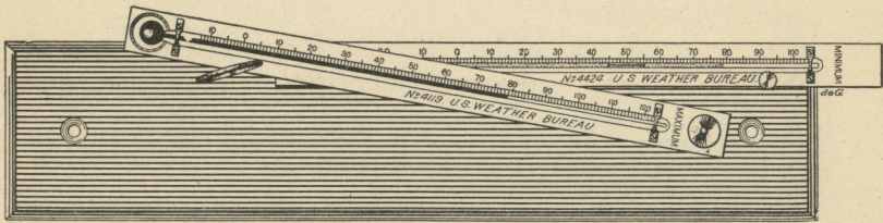
FIG. 3.—Maximum and minimum thermometers on old style board support.
