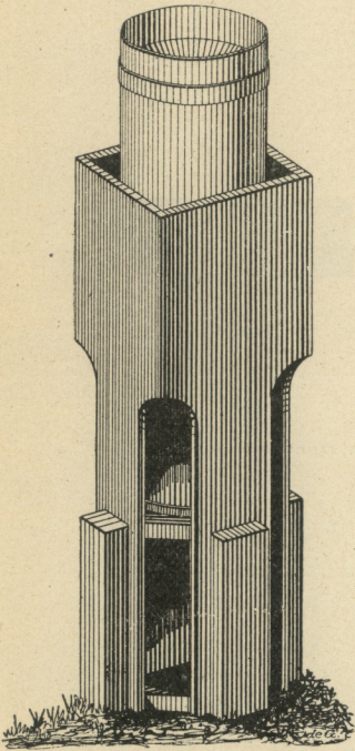
FIG. 12.—Rain gage and support.
