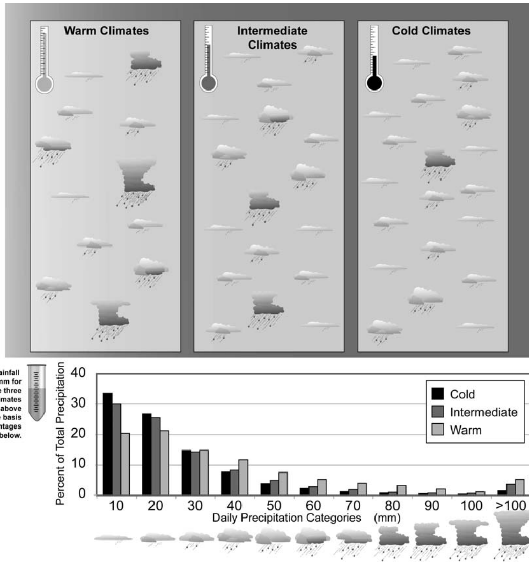
FIGURE 2-11 The diagram shows that warmer climates have a higher percentage of total rainfall coming from heavy and very heavy events. The data are based on a worldwide distribution of observing stations, each with the same seasonal mean precipitation amount of 230 (±5) mm. In cool climates, there are more daily precipitation events than in warmer climates (adapted from Karl and Trenberth 2003). The various cloud and rain symbols reflect the different daily precipitation rates and are categorized in the top panel of this figure to reflect the approximate proportion of the different rates for cool, moderate, and warm climates across the globe.
