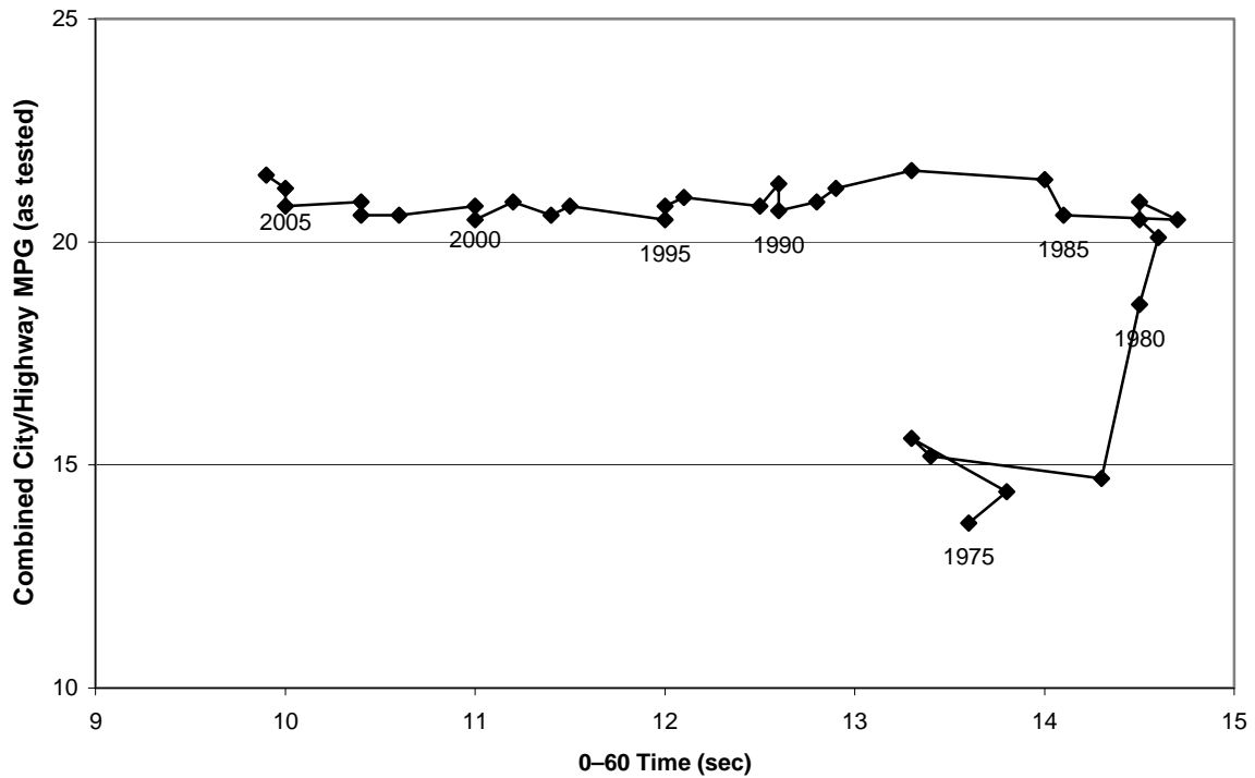
FIGURE B-8b Truck 55/45 laboratory MPG versus 0-60 time by model year. (Source: Heavenrich 2006, Figure 7, p. 16.)
