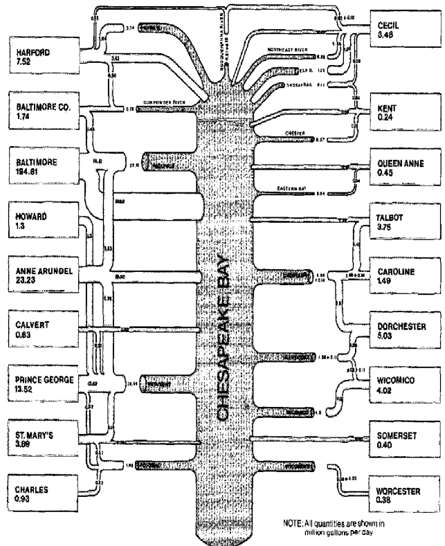
FIGURE 10 WASTEWATER DISCHARGE DIAGRAM
