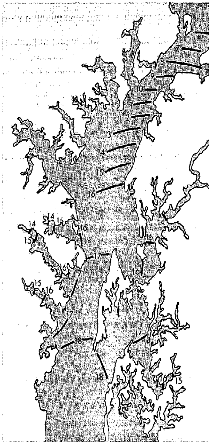
Effect of Susquehanna River discharges on surface salinity values in the spring (high flows) and fall (low flows) in 1964. Lines represent equal salinity observations in parts per thousand (p.p.t.).
