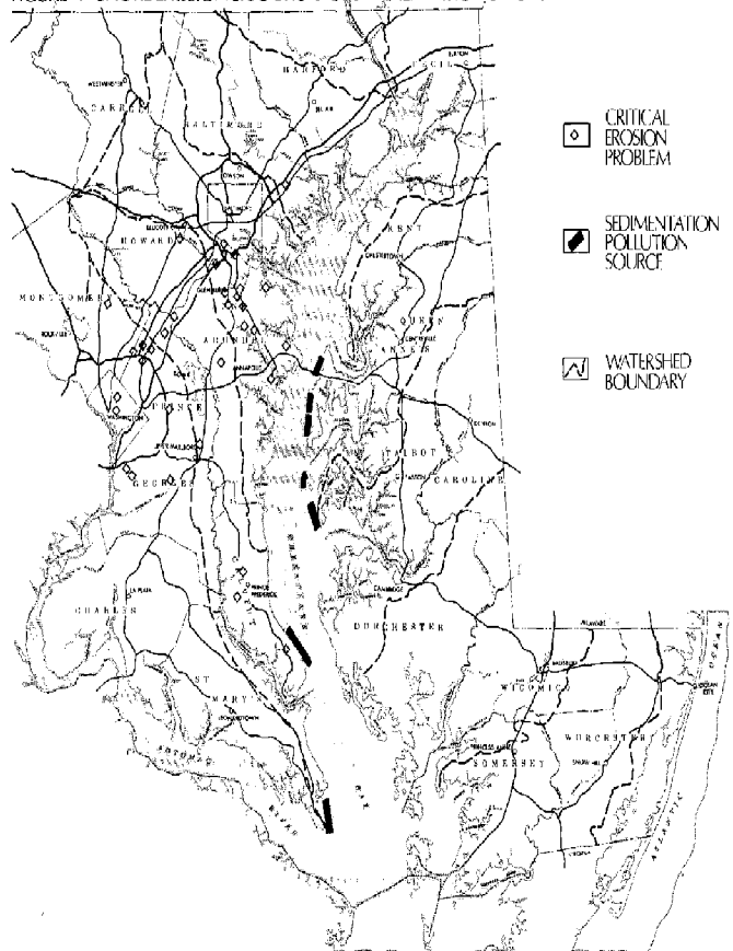
FIGURE 19 SHORE EROSION & SOURCES OF SEDIMENTATION & TURBIDITY
