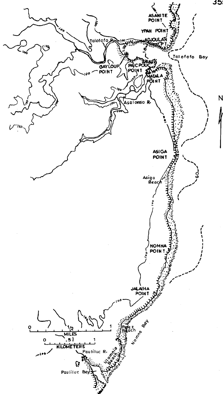
Figure 168b. Map showing the 100 foot coastal contour (solid line), rocky shorelines, cut benches, beach deposits, alluvium, fringing reef-flat platforms (stippled region seaward of shorelines), reef margin, and the 18 foot (solid line) and 60 foot (dashed line) submarine contour lines for Sector XII from Talofoto Bay to Pauliluc Bay. See Figures 168a and 168c for the remainder of Sector XII (map legend on 168a).
