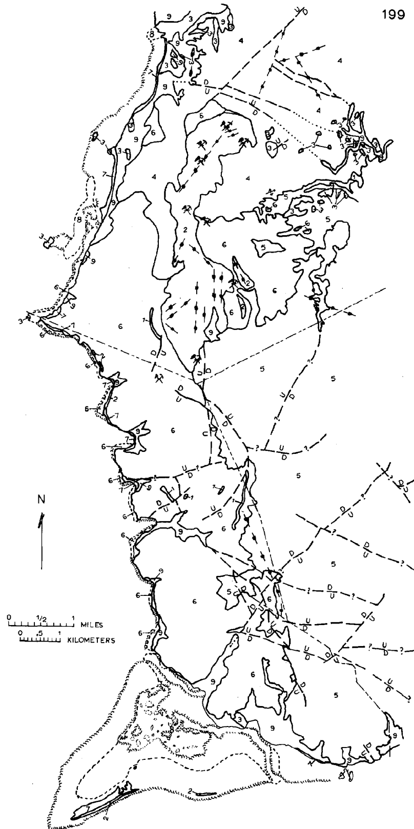
Figure 12d. Engineering geology map for most of Sector X (see 12c for northern part), the southern tip of Sector XII, and Sector XI. A map legend and explanation for the geology map units (1-9) is given on pages 193-195. To be used in conjunction with Tables 5 and 6 (pages 373-376). Map modified from Tracey et al. (1959).
