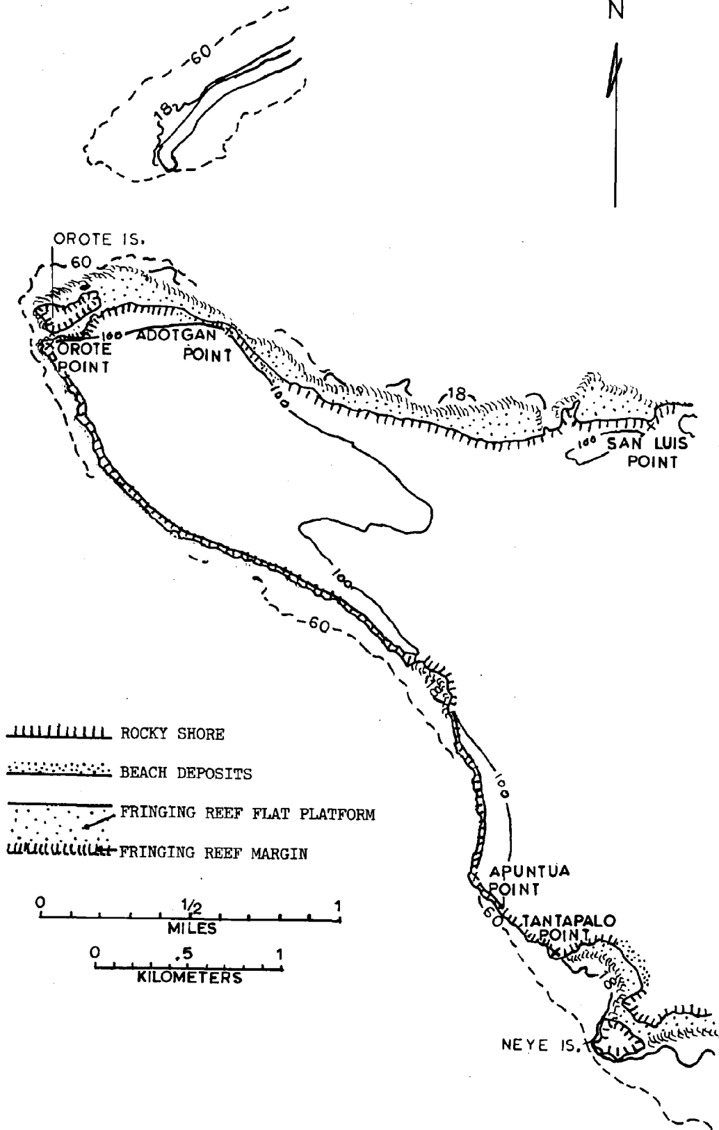
Figure 136. Map showing the 100 foot coastal contour (solid line), rocky shorelines, beach deposits, fringing reef-flat platforms (stippled region seaward of shoreline), reef margin, and the 18 foot (solid line) and 60 foot (dashed line) submarine contour lines for Sector IX.
