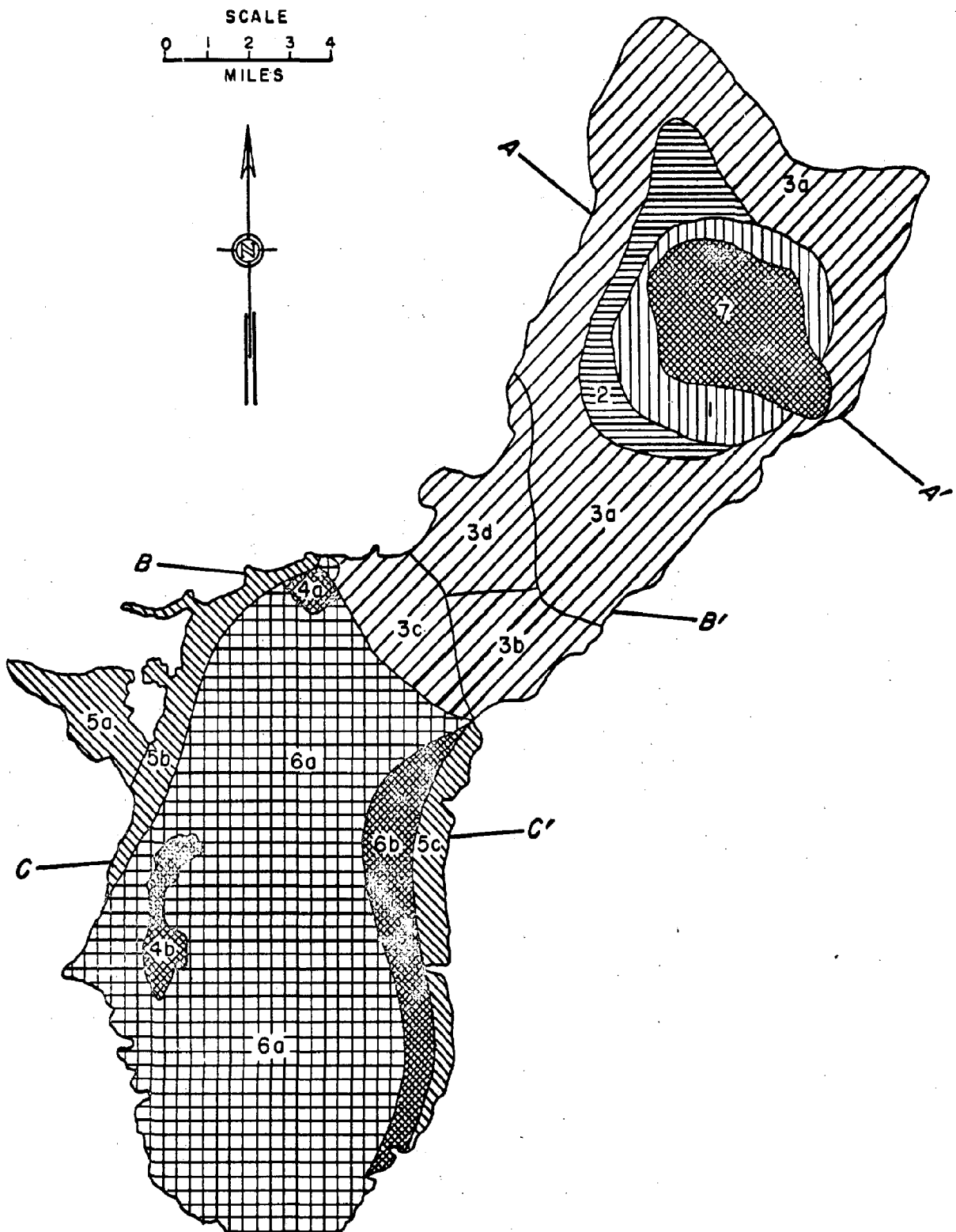
Figure 13. Map showing ground-water areas in Guam, and the locations of geologic sections shown in Figure 14. An explanation legend is given on the two preceding pages. Figure taken from Ward and Brookhart (1962).
