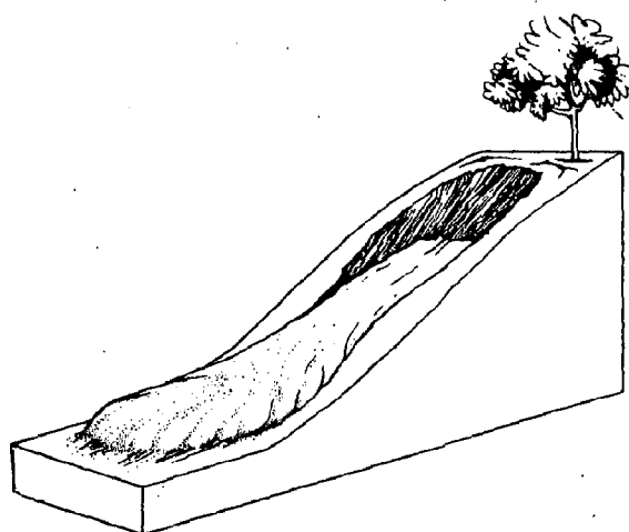
D Earthflow : soil and other colluvial materials that move downslope in a manner similar to a viscous fluid.
