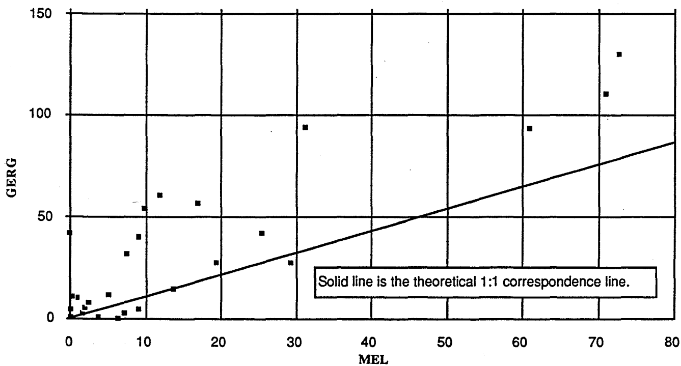
FIGURE 5. IMW NOAA-NIST Mussel Tissue IV Intercalibration (QA92TiS4) Compare all Chlorobiphenyl and Chlorinated Pesticide Data as ng/gdw
