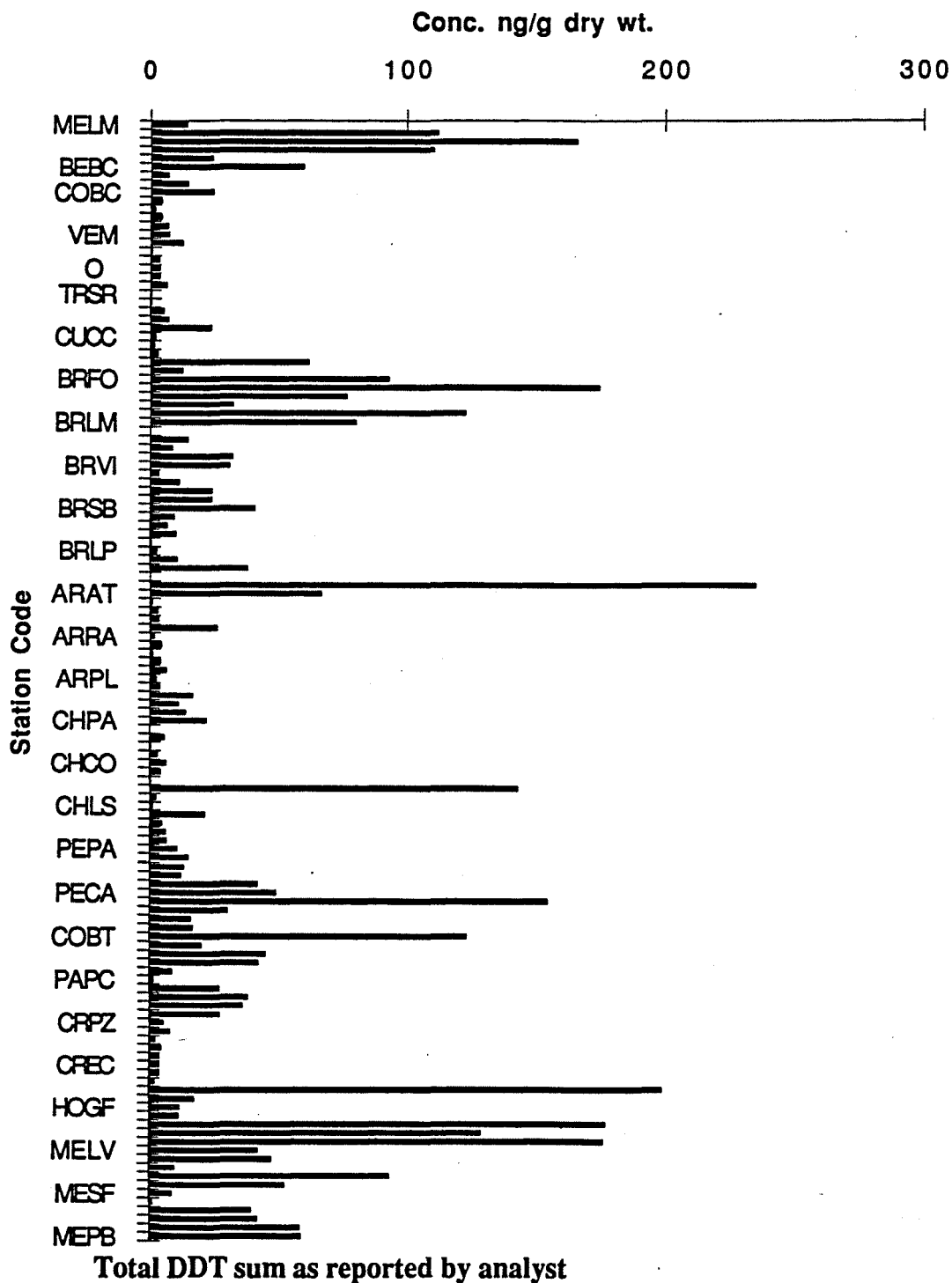
FIGURE 17. Total DDT Concentration South and Central America
