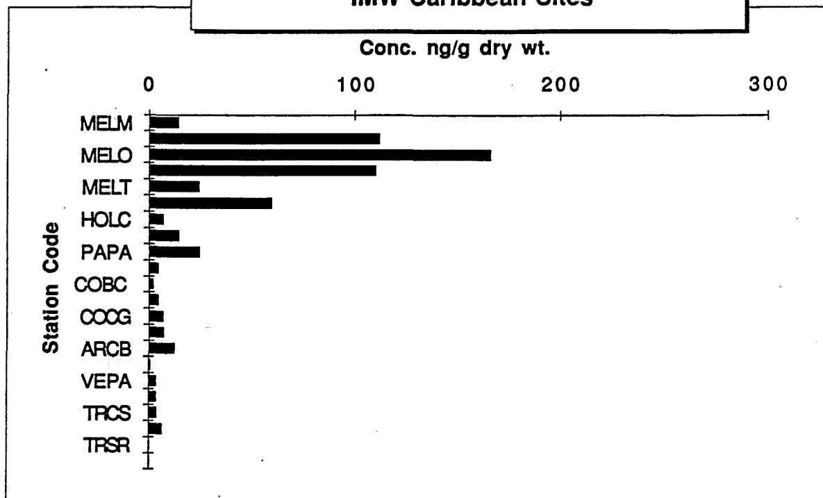
FIGURE 19. Total DDT Concentration IMW Caribbean Sites
