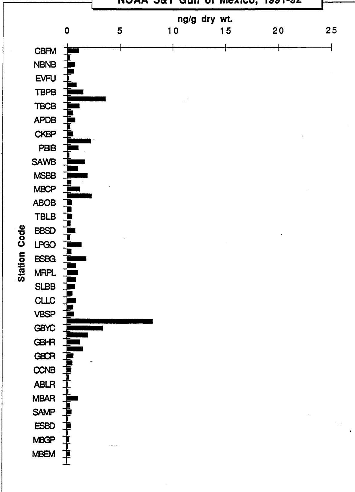
FIGURE 23. Lindane Concentration NOAA S&T Gulf of Mexico, 1991-92
