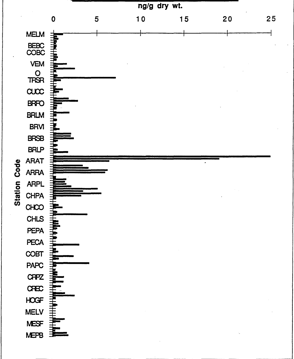
FIGURE 22. Lindane Concentration South and Central America
