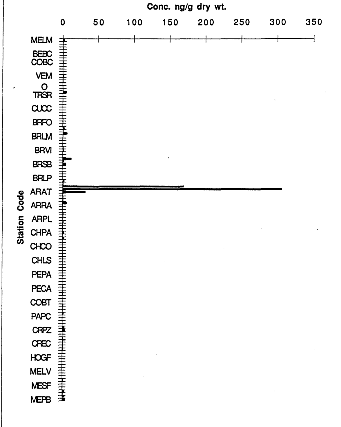
FIGURE 24. Gamma Chlorane Concentration South and Central America
