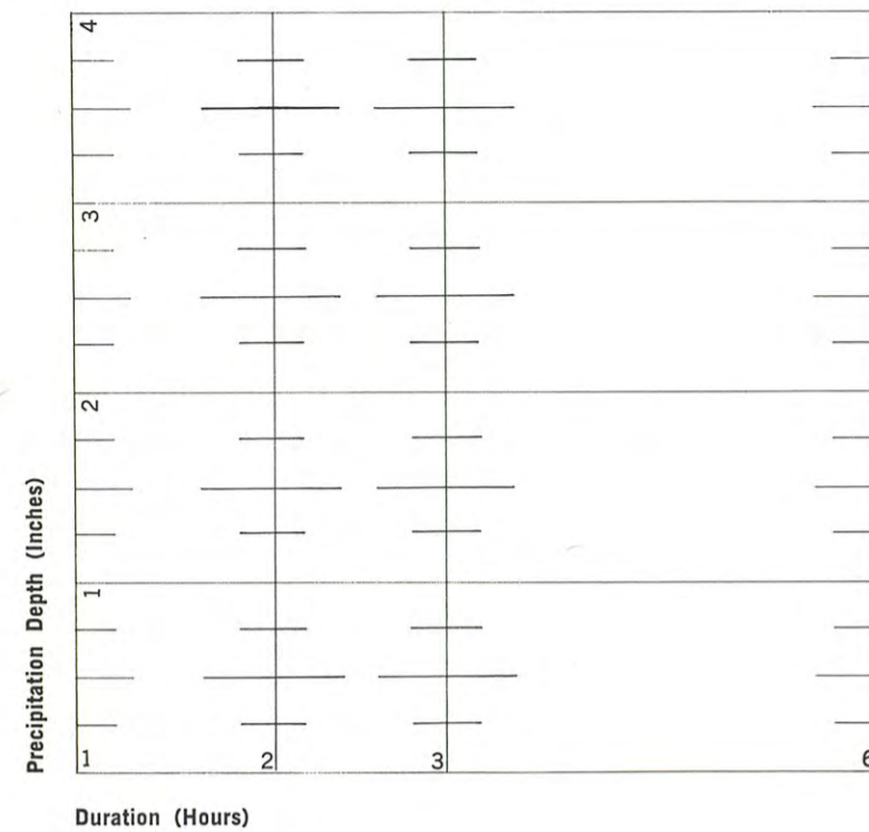
Figure 16. Precipitation depth-duration diagram (1 to 6 hrs).
