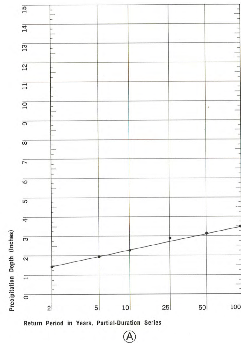
Figure 18. Illustration of use of precipitation-frequency diagrams using values from precipitation-frequency maps and relations at 47°00' N., 110°00' W.
