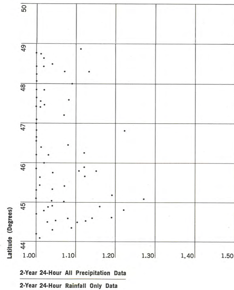
Figure 15. Ratio of 2-yr 24-hr precipitation values based on all precipitation data series to values from rainfall only data series—Montana and northern Wyoming.
