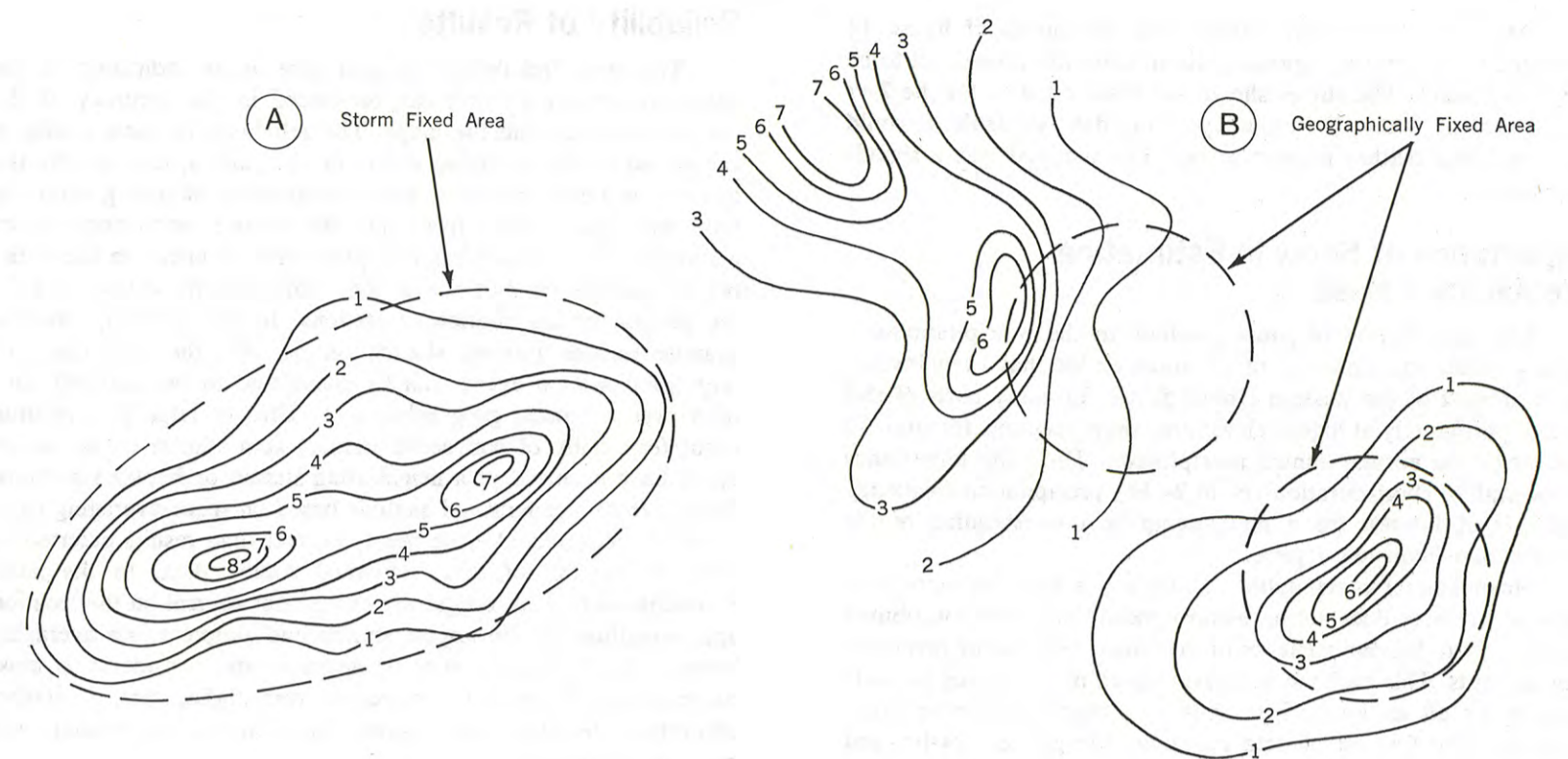
Figure 13. Examples of (A) isohyetal pattern centered over basin as would be the case for storm-centered depth-area curves and (B) two possible occurrences of isohyetal patterns over a geographically fixed area as would be the case in development of curves for a geographically fixed area.
