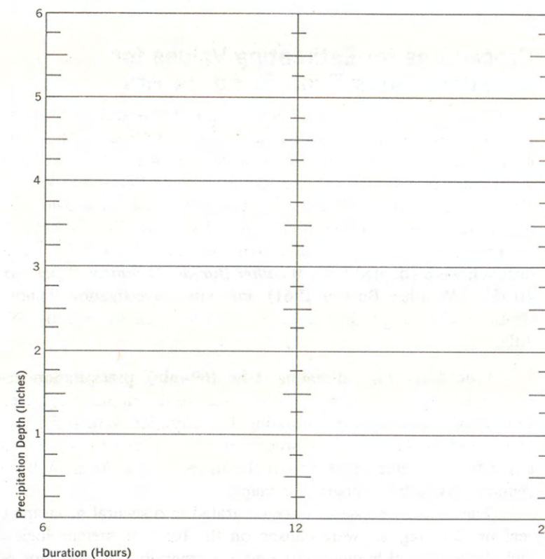
Figure 17. Precipitation depth-duration diagram (6- to 24-hr).
