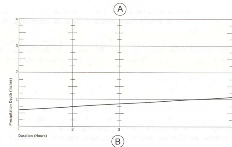
Figure 18. Illustration of use of precipitation-frequency diagrams using values from precipitation-frequency maps and relations at 43°00' N., 109°00' W.
