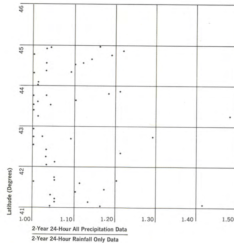
Figure 15. Ratio of 2-yr 24-hr value for all data to 2-yr 24-hr value for rainfall only vs. latitude.
