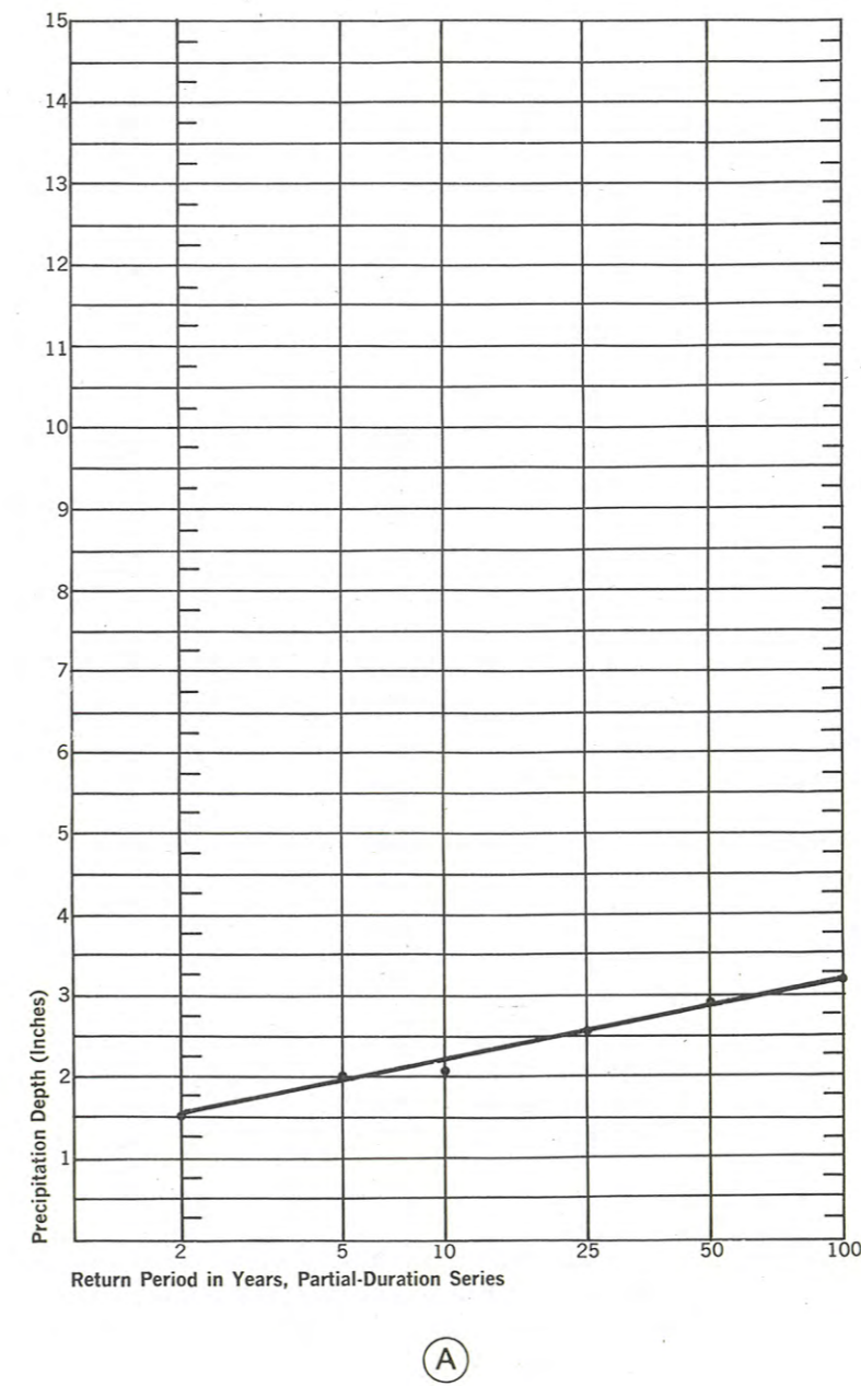
Figure 17. Illustration of use of precipitation-frequency diagrams using values from precipitation-frequency maps and relations.
