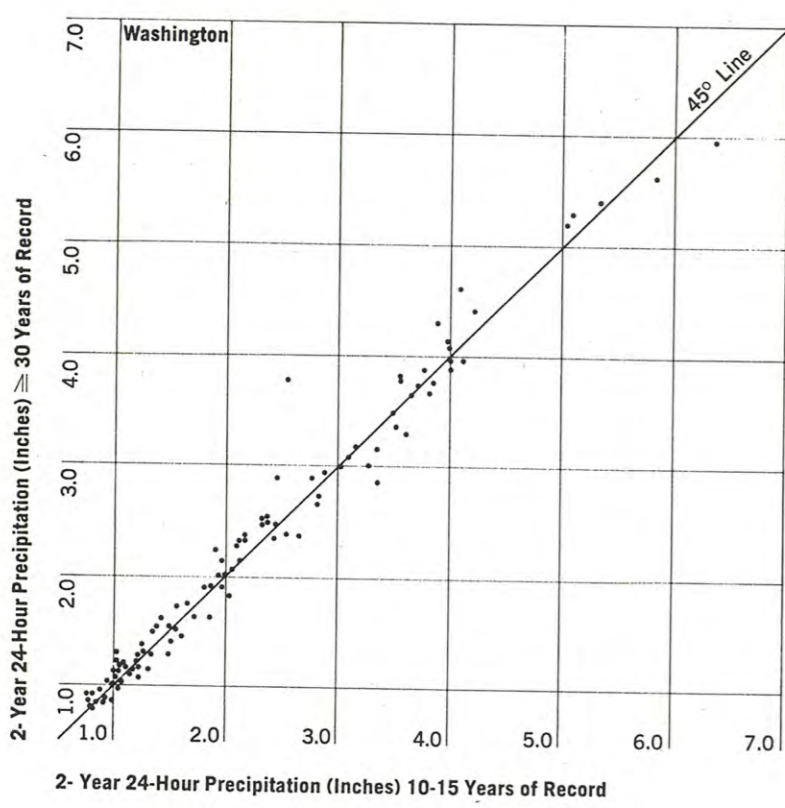
Figure 2. Test of 2-yr 24-hr precipitation values from short- and long-record stations for the State of Washington.
