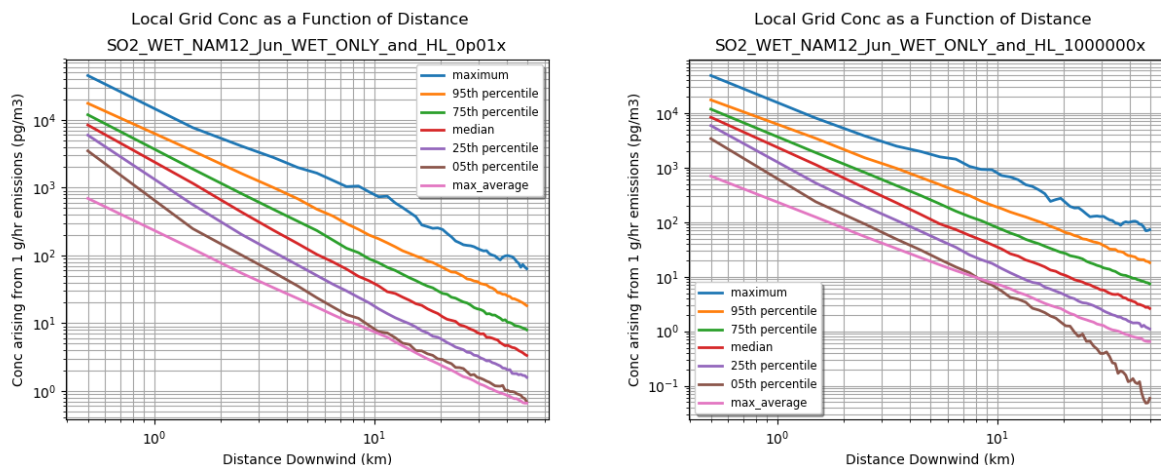
Figure 75. Local grid summary of statistical distribution of hourly concentration values using HLC for wet-deposition 0.01x (left) and 10 6 x (right) the nominal value for SO 2 (June 2017, NAM-12km meteorological data).
