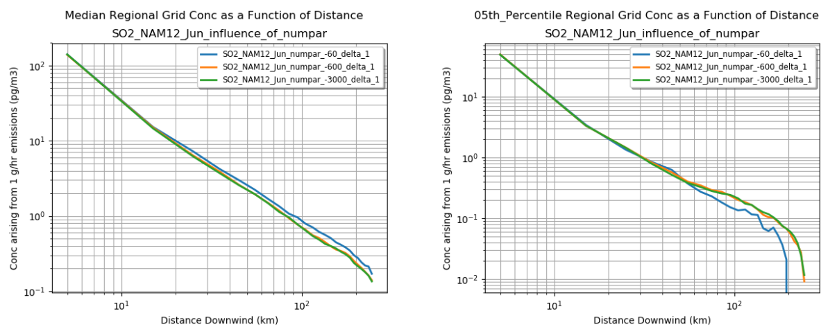
Figure 27. Influence of NUPAR on Regional Grid Results
