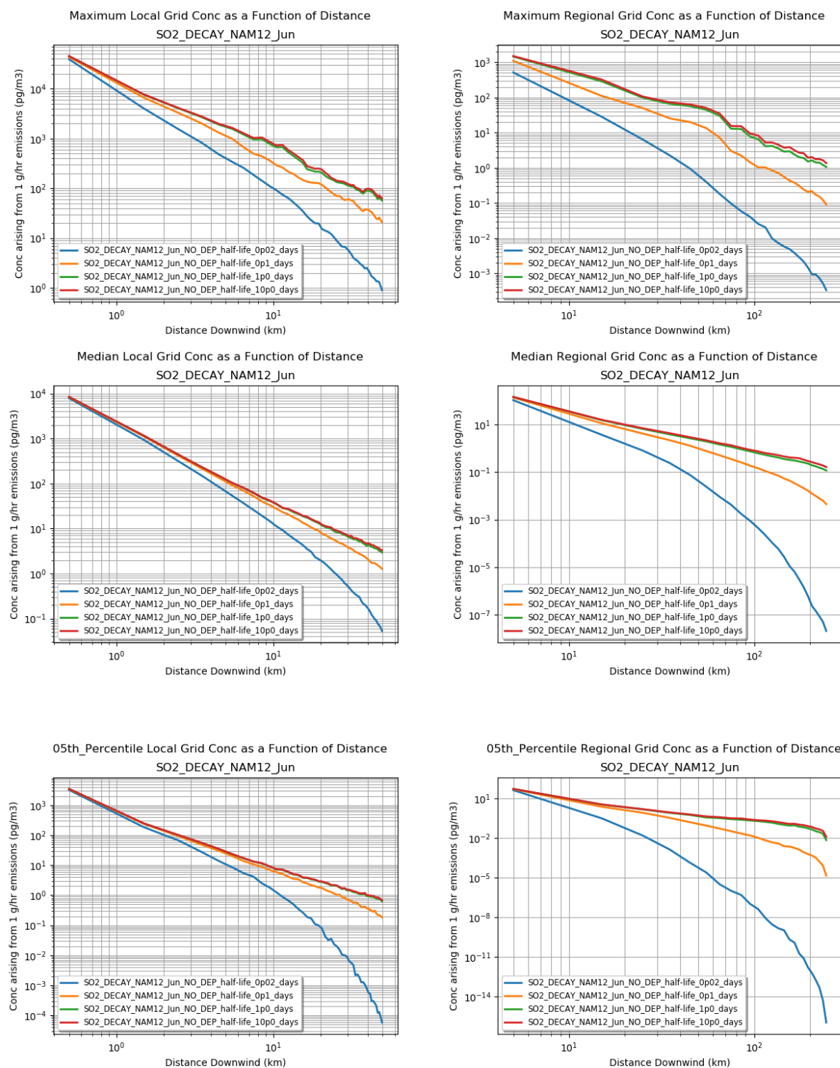
Figure 89. Influence of chemical transformation half-life on maximum (top), median (middle) and 5th percentile (bottom) hourly SO 2 concentrations simulated for local (left) and regional (right) grids. 4-week simulation for June 2017, NAM-12km meteorological data.
