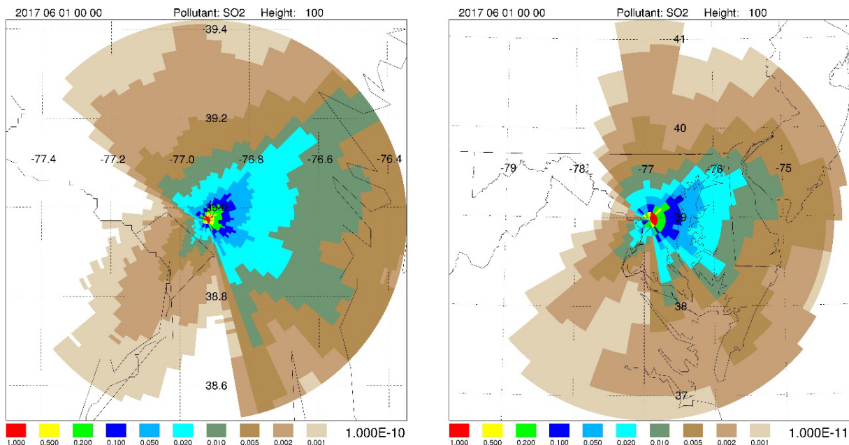
Figure 11. Illustrative average concentrations (g/m 3 ) in 0-100 m layer over 4-week simulation for local grid (left) and regional grid (right) (June 2017, WRF-27km meteorological data).
