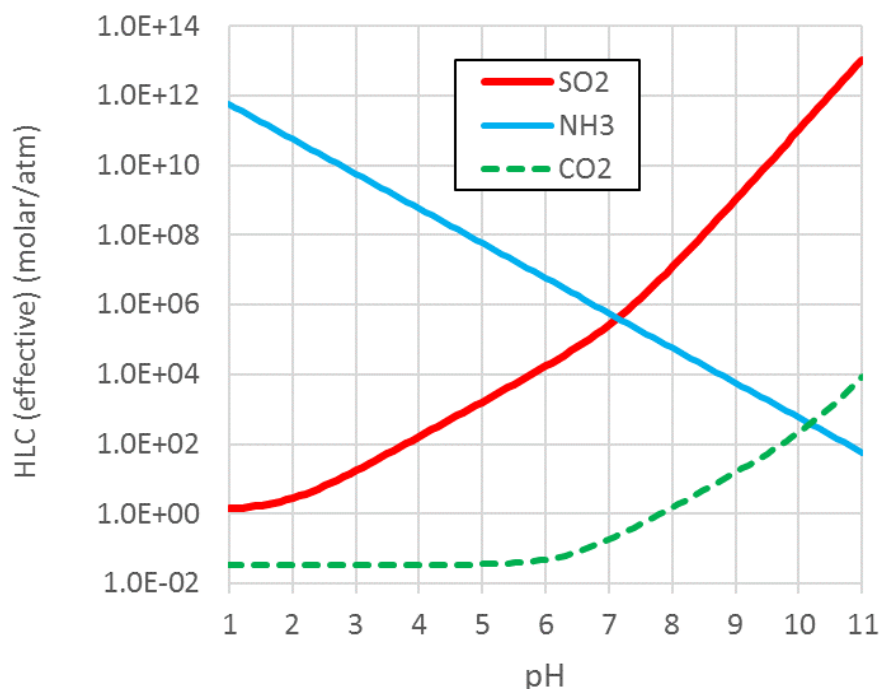
Figure 63. Effective Henry's Law Constant for SO 2 , NH 3 , and CO 2 at 298 K as function of pH.
