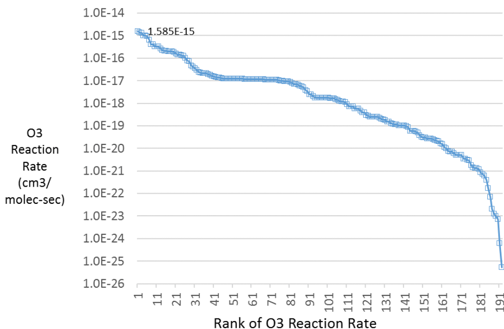
Figure 94. Estimated or Experimental Reaction rate with Ozone for ALOHA Chemicals.
