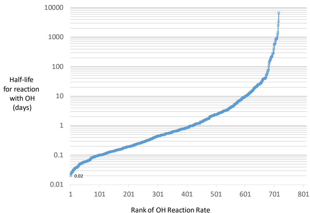
Figure 88. Estimated half-life (days) for reaction with Hydroxyl Radical for ALOHA Chemicals. Assumes [OH] = 1.5 \times 10^6 molecules / cm^3 . Hydroxyl radical reaction rates could only be estimated for ~700 ALOHA chemicals.
