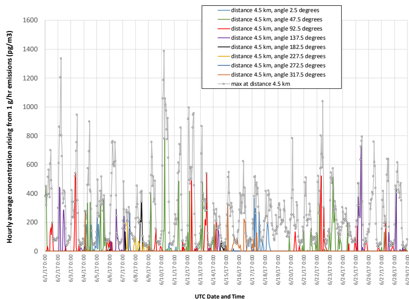
Figure 13. Hourly concentrations 4.5 km from source at different angular orientations, and maximum concentrations at each time at any angular orientation
