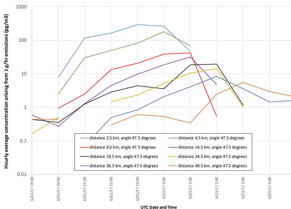
Figure 10. Using NAM12 Meteorological Data: Hourly concentrations at an angular orientation of 47.5 degrees at different distances from the source (expanded view for a shorter time period, with a logarithmic concentration scale).
