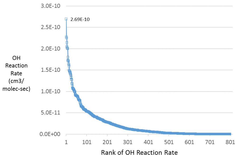
Figure 86. Estimated Reaction rate with HYDROXL Radicals for ALOHA Chemicals.
