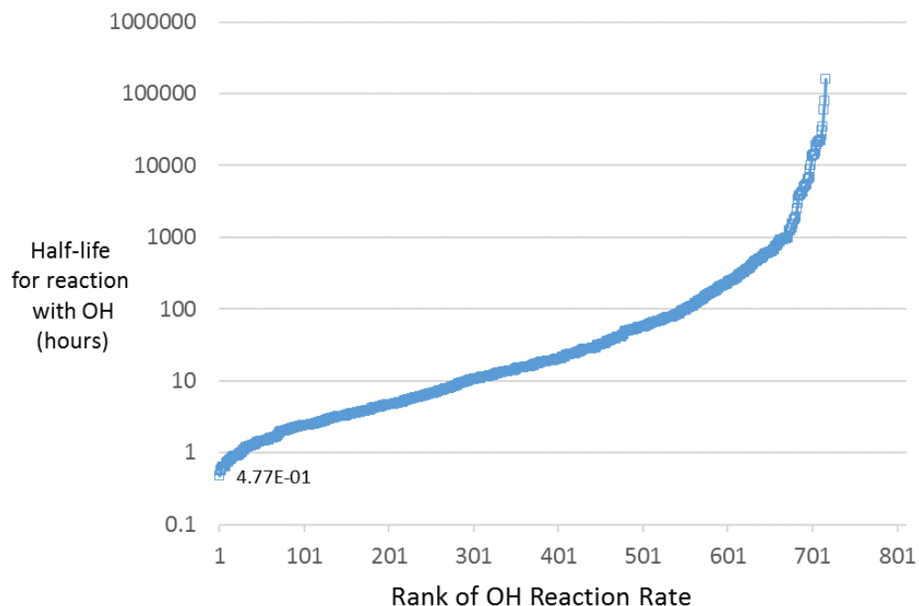
Figure 87. Estimated half-life (hours) for reaction with Hydroxyl Radical for ALOHA Chemicals. Assumes [OH] = 1.5 \times 10^6 molecules / cm^3 . Hydroxyl radical reaction rates could only be estimated for ~700 ALOHA chemicals.
