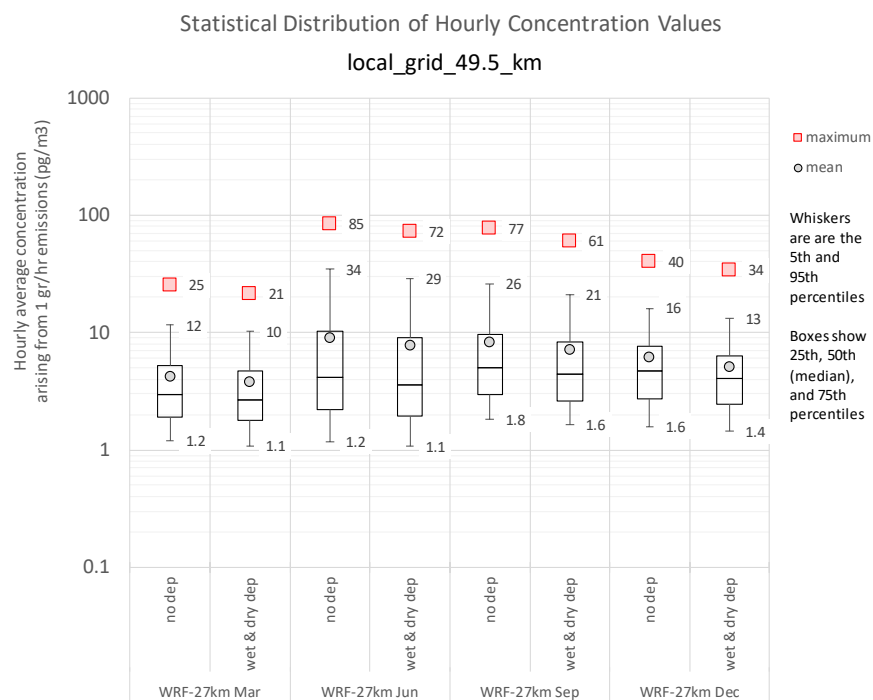
Figure 36. Statistical distribution of hourly maximum concentrations on local grid at a distance of 49.5 km. NAM-12km (top) and WRF-27km (bottom) simulations with no deposition vs. those with wet and dry deposition (with default parameters) for SO 2 . No chemical transformation included.
