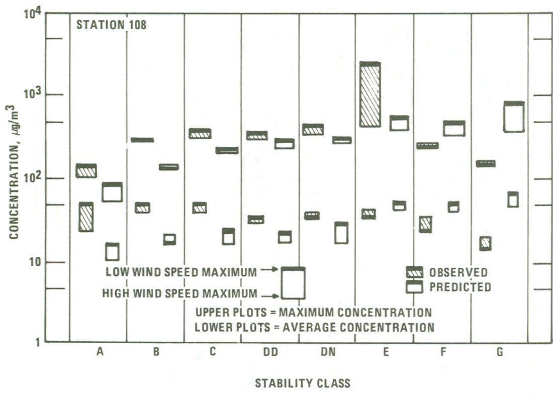
Figure 3. Maximum and average \text{SO}_2 concentrations for each stability wind speed category for station 108.
